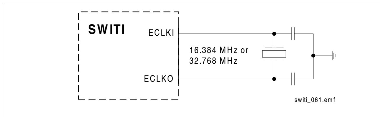
Figure 41 External Crystal
