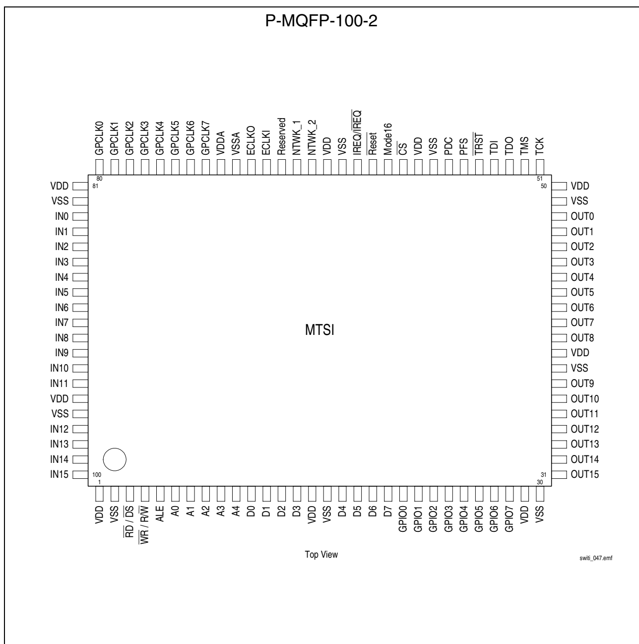
Figure 3 Pin Configuration
