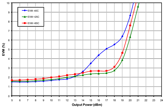
Figure 22: Tx Path Dynamic EVM vs. Output Power Across Temperature (Freq = 5.5 GHz, V cc = +3.3 V, 802.11a, 54 Mbps OFDM)
