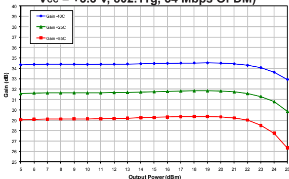
Figure 5: Tx Path Gain vs. Output Power Across Temperature (Freq = 2.45 GHz, V_{CC} = +3.3\text{ V} , 802.11g, 54 Mbps OFDM)
