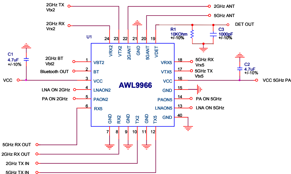
Figure 40: Application Circuit
