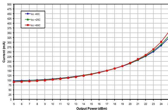
Figure 8: Tx Path Icc vs. Output Power Across Temperature (Freq = 2.45 GHz, V_{CC} = +3.3\text{ V} , 802.11g, 54 Mbps OFDM)
