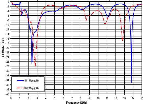
Figure 13: 2 GHz Tx Path S11 & S22 Return Loss ( T_c = +25\text{ }^\circ\text{C} , V_{CC} = +3.3\text{ V} )
