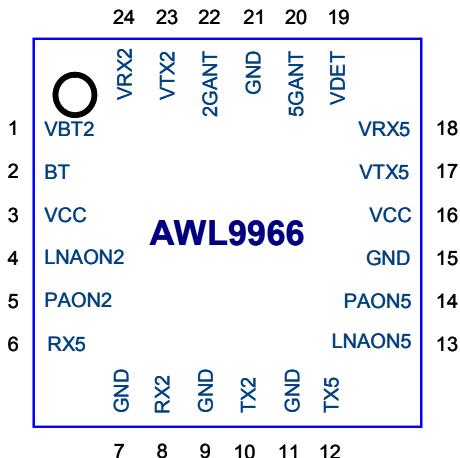
Figure 2: Pinout Diagram
