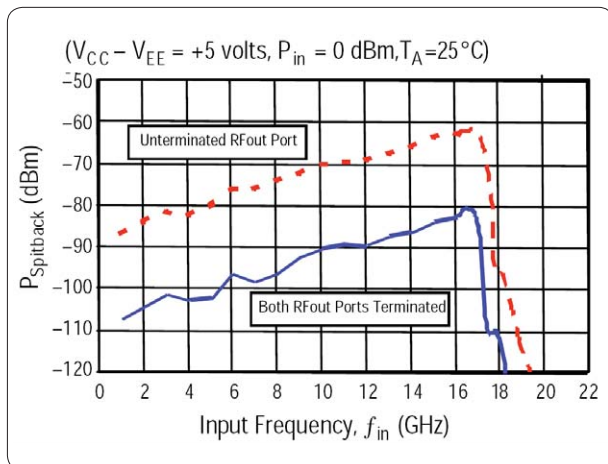
Figure 8. Typical "Spitback" power P(f_{\text{out}}) appearing at RF input port
