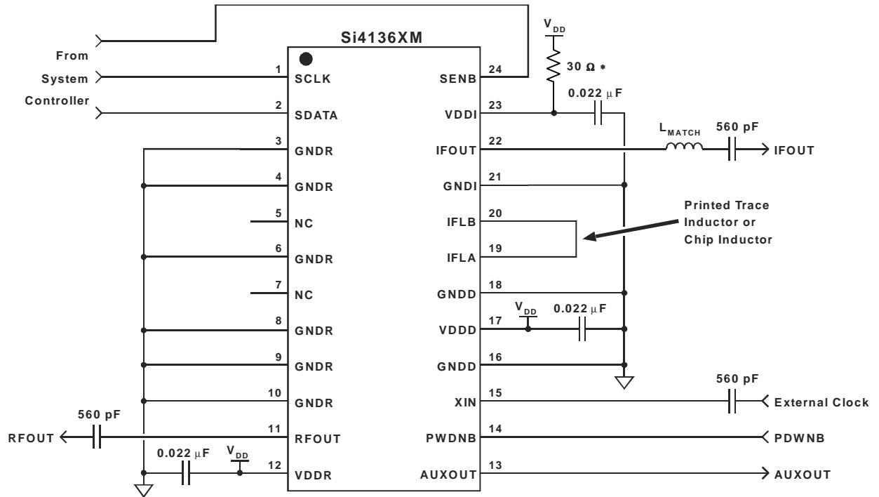
Figure 13. Typical Application Circuit: Si4136XM-BT
