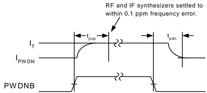
Figure 5. Hardware Power Management Timing Diagram
