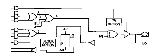
Figure 3c. Combinatorial Output, Combined Terms
