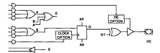
Figure 2b. Registered Output, Separate Terms
