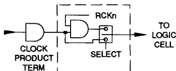
Figure 5. Clock Option
