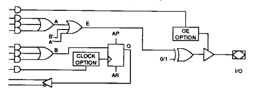
Figure 3d. Combinatorial Output, Separate Terms
