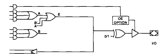
Figure 2d. Combinatorial Output, Separate Terms
