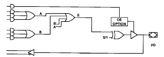
Figure 4c. Combinatorial Output, Combined Terms
