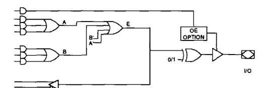
Figure 2c. Combinatorial Output, Combined Terms
