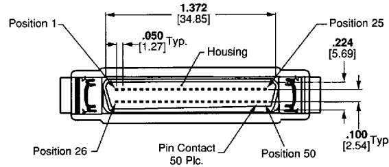
"A" Cable Single-Ended, Active Part No. 869912-1
