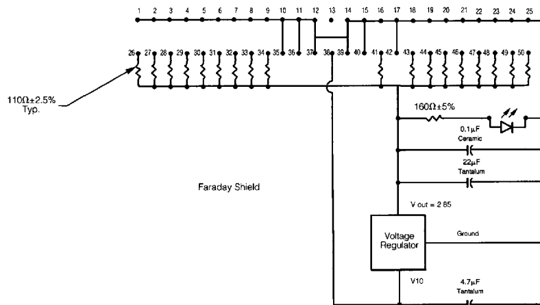
"A" Cable Single-Ended, Active Part No. 869912-1
