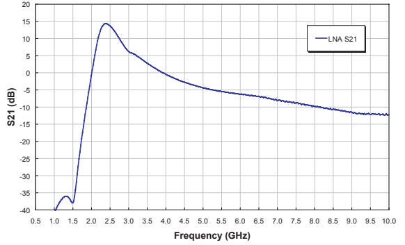
Figure 21: Rx Path S21 Response ( V_{CC} = +3.6\text{ V} , T_A = 25^\circ\text{C} )
