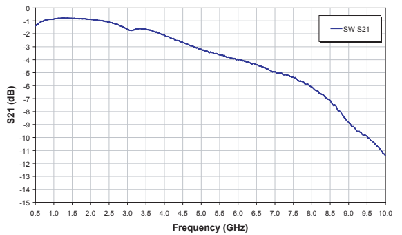
Figure 23: Bluetooth Path S21 Response ( V_{CC} = +3.6\text{ V} , T_A = 25^\circ\text{C} )
