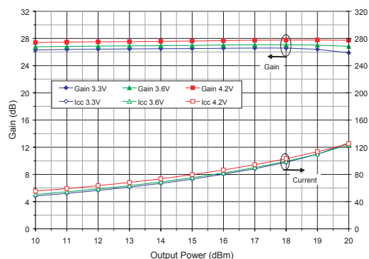
Figure 12: Gain and I_{CC} vs. Output Power Across Power Supply Voltage (Freq = 2.45 GHz, T_A = 25^\circ\text{C} )
