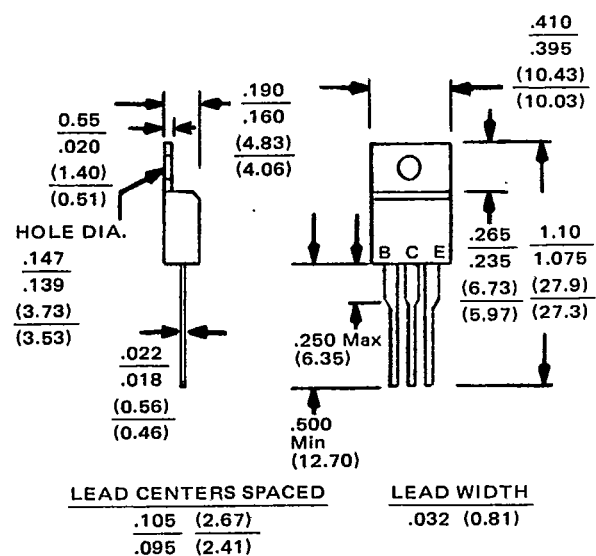
To-220AB
