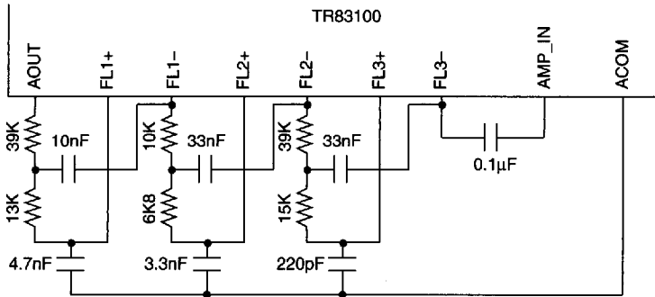
Figure 4 • Active Filter Connections
