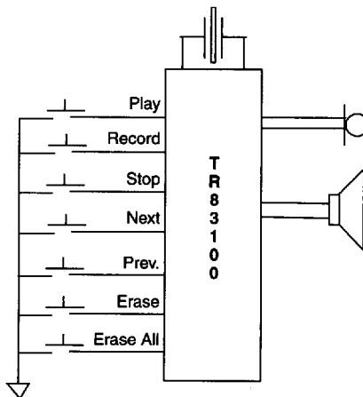
Figure 3 • Switch Functions
