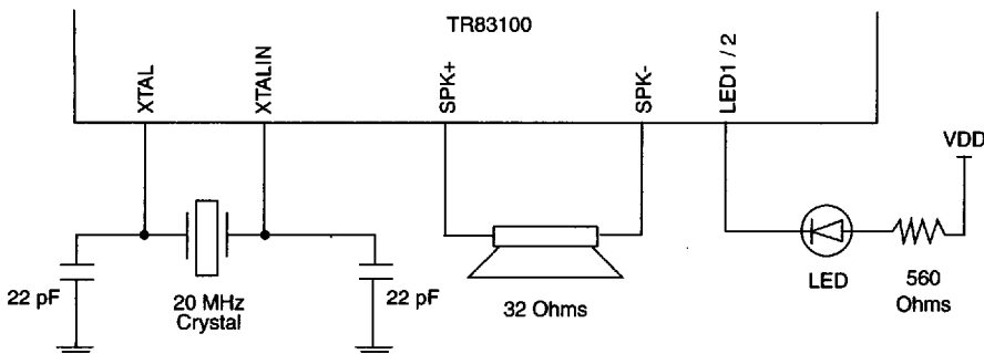
Figure 5 • Crystal, Speaker & LED connections
