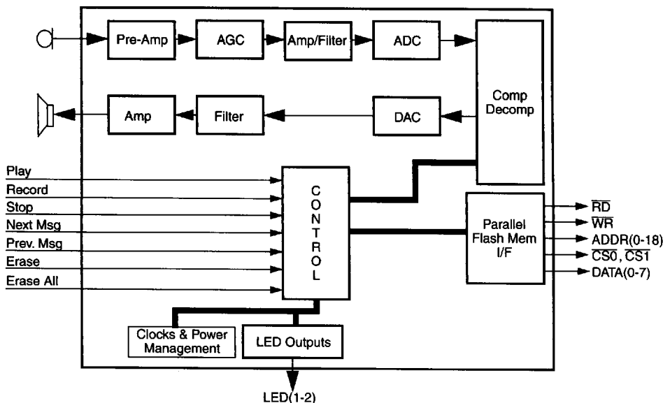
Figure 1 • TR83100 Voice Storage Controller
