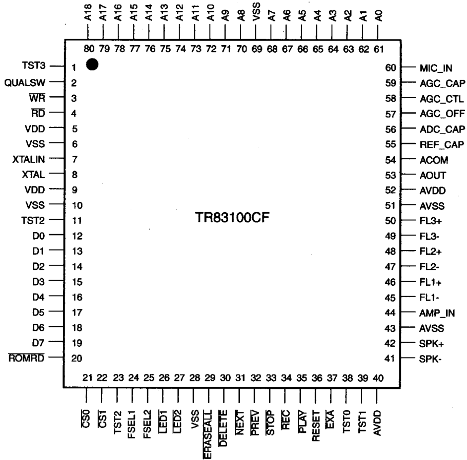
Figure 2 • Package Pin Layout, Top View
