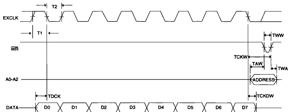
WRITE TIMING DIAGRAM (SERIAL VERSION)
