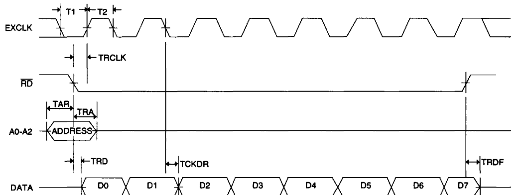
READ TIMING DIAGRAM (SERIAL VERSION)
