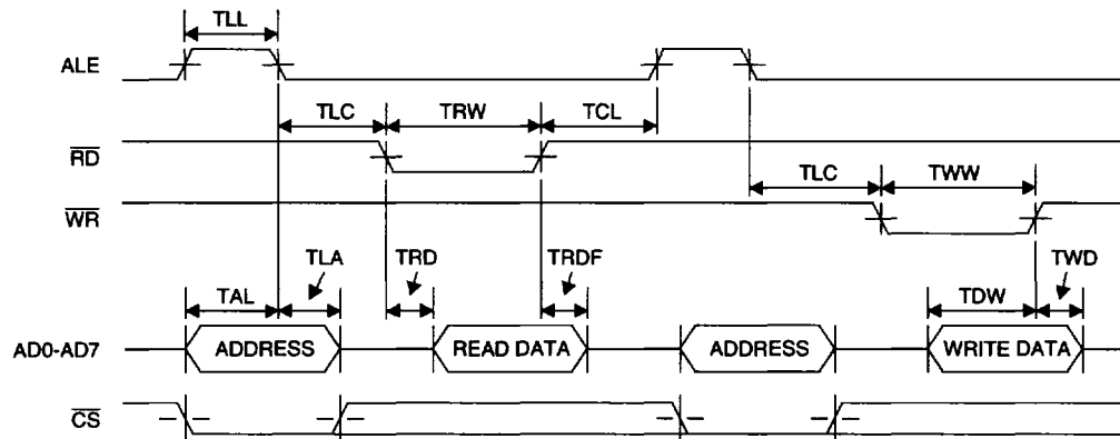
BUS TIMING DIAGRAM (PARALLEL VERSION)
