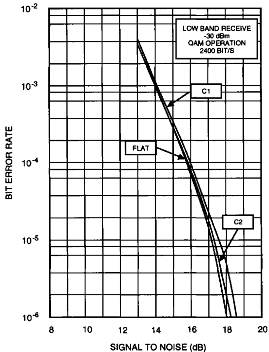
TSC 73K224L BER vs S/N-QAM-LOW BAND
