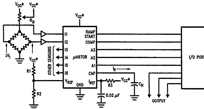
FIGURE 9. Ratiometric Strain Gage Sensor/Controller
