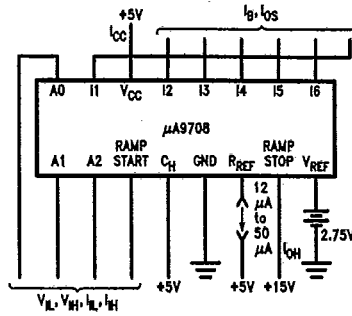
FIGURE 4. Static Measurements
