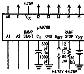
FIGURE 3. Linearity/Acquisition Time/Conversion Time Test Circuit
