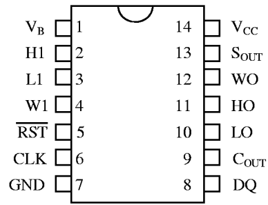
14-Pin DIP (300-mil) See Mech. Drawings Section
