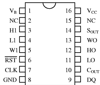
16-Pin SOIC (300-mil) See Mech. Drawings Section
