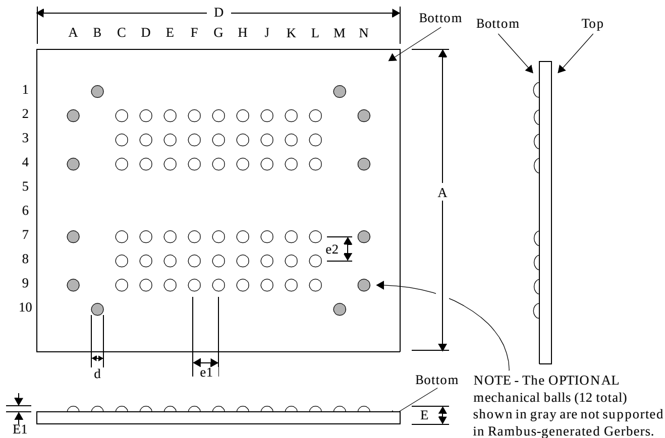
Figure 63: Center-Bonded uBGA Package
