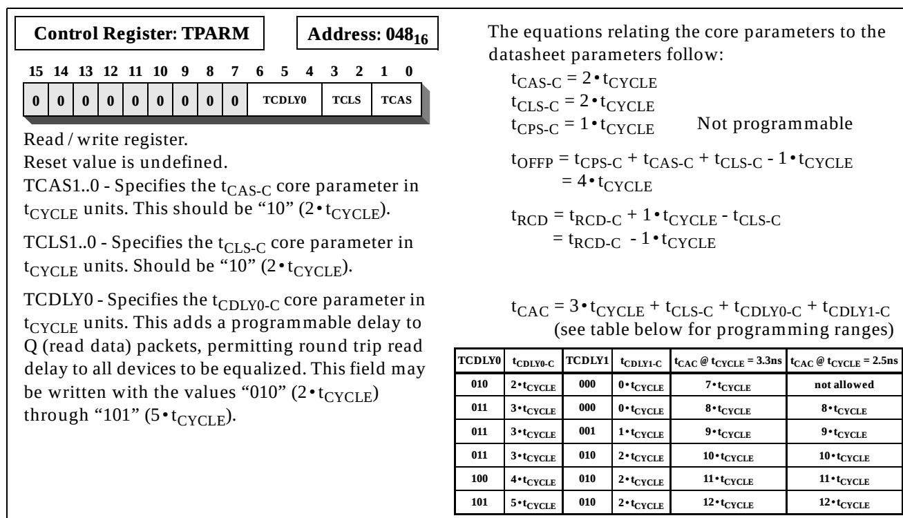
Figure 39: TPARM Register
