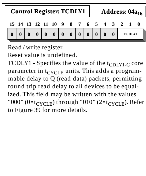
Figure 41: TCDLY1 Register
