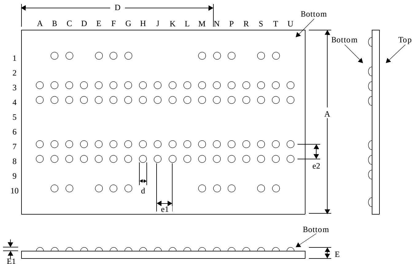
Figure 62: Center-Bonded uBGA Package
