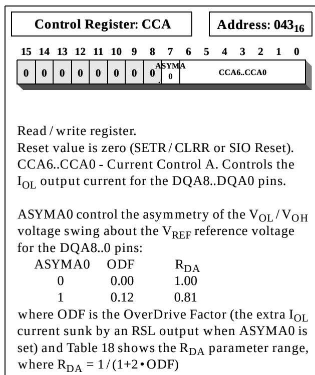
Figure 33: CCA Register
