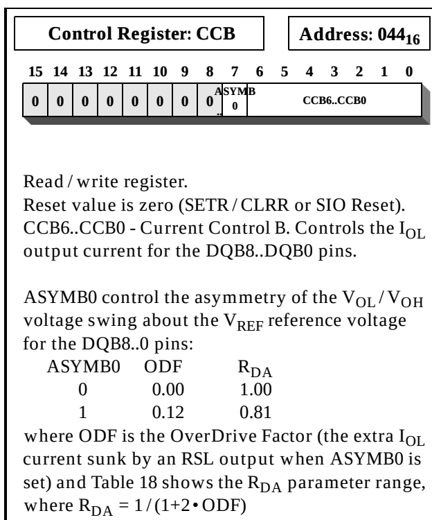
Figure 35: CCB Register
