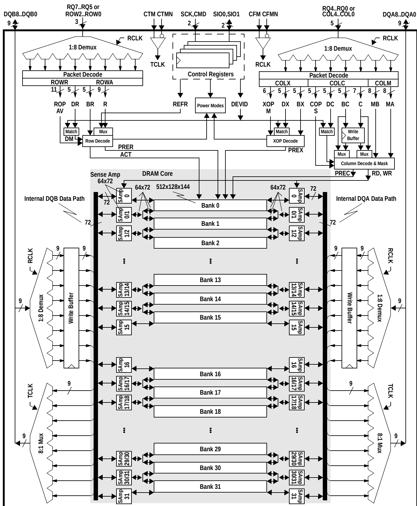
Figure 2: 256/288-Mbit (512Kx16/18x32s) Direct RDRAM Block Diagram
