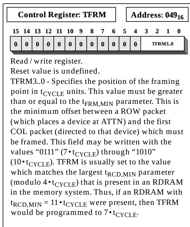
Figure 40: TFRM Register
