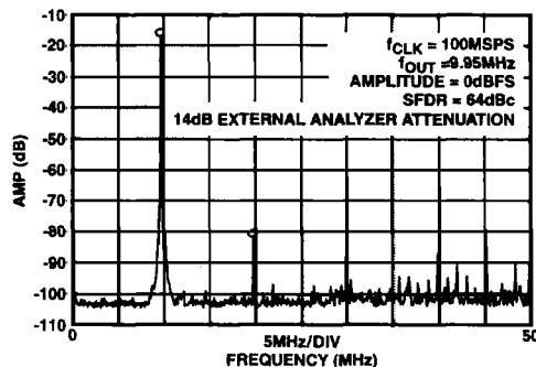
FIGURE 12. SINGLE TONE SFDR
