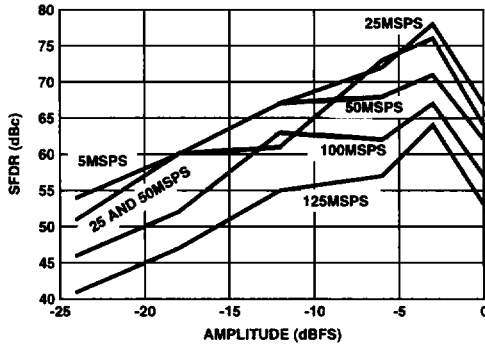
FIGURE 26. SFDR vs AMPLITUDE, f_{CLK}/f_{OUT} = 5
