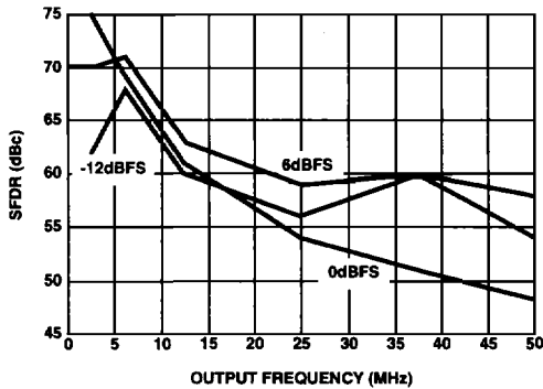
FIGURE 5. SFDR vs f_{OUT} , CLOCK = 125MSPS
