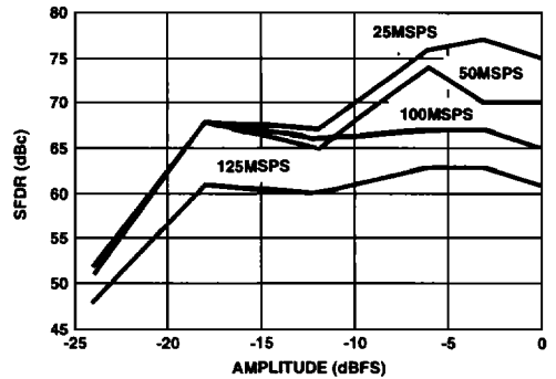
FIGURE 6. SFDR vs AMPLITUDE, f_{CLK}/f_{OUT} = 10
