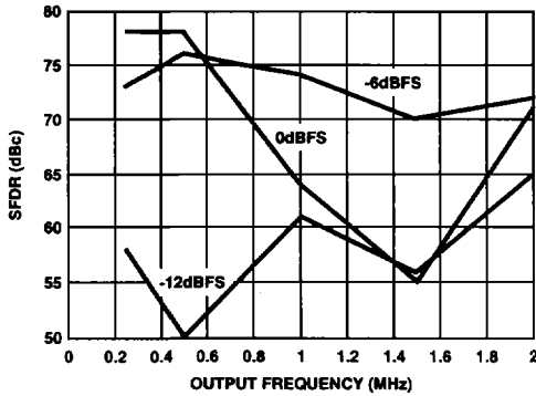
FIGURE 1. SFDR vs f_{OUT} , CLOCK = 5MSPS
