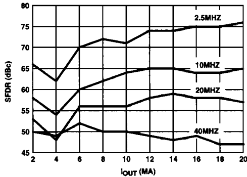
FIGURE 28. SFDR vs I_{OUT} , CLOCK = 100MSPS
