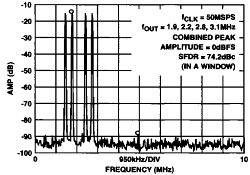
FIGURE 35. FOUR-TONE, CLOCK = 50MSPS
