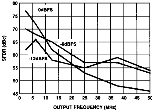
FIGURE 24. SFDR vs f_{OUT} , CLOCK = 125MSPS
