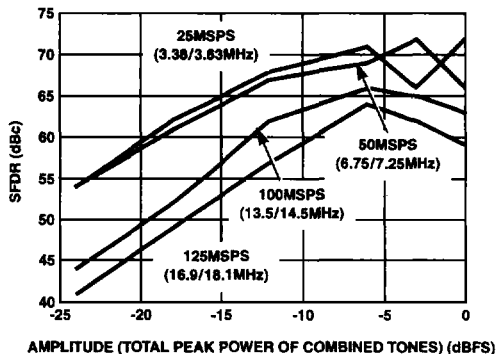
FIGURE 8. SFDR vs AMPLITUDE OF TWO TONES, f_{CLK}/f_{OUT} = 7
