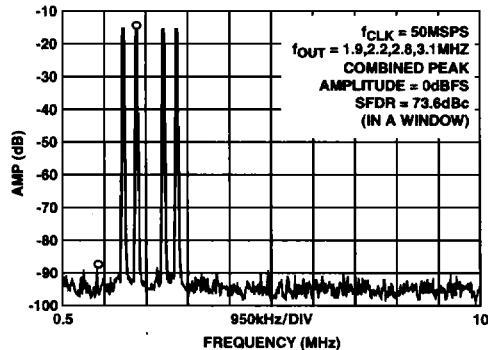
FIGURE 16. FOUR-TONE, CLOCK = 50MSPS
