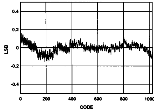
FIGURE 18. INTEGRAL NONLINEARITY
