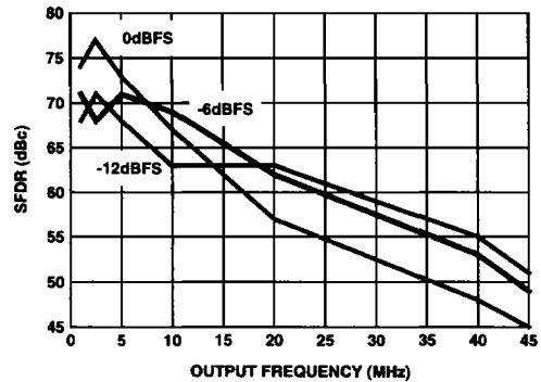
FIGURE 23. SFDR vs f_{OUT} , CLOCK = 100MSPS
