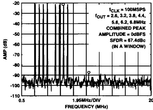
FIGURE 34. EIGHT-TONE, CLOCK = 100MSPS
