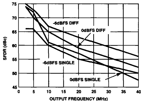
FIGURE 10. DIFFERENTIAL vs SINGLE-ENDED, CLOCK = 100MSPS
