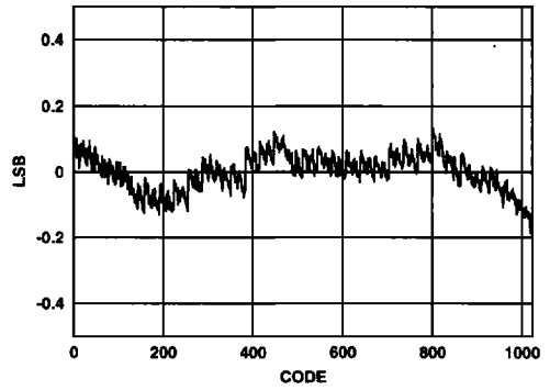
FIGURE 37. INTEGRAL NONLINEARITY
