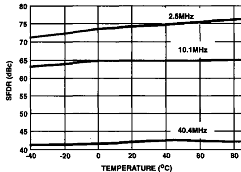
FIGURE 11. SFDR vs TEMPERATURE, CLOCK = 100MSPS
