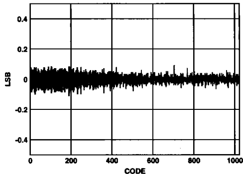
FIGURE 17. DIFFERENTIAL NONLINEARITY
