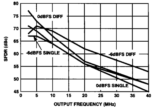
FIGURE 29. DIFFERENTIAL vs SINGLE-ENDED, CLOCK = 100MSPS
