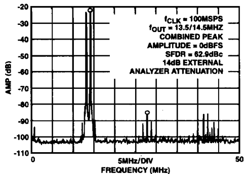
FIGURE 13. TWO-TONE, CLOCK = 100MSPS
