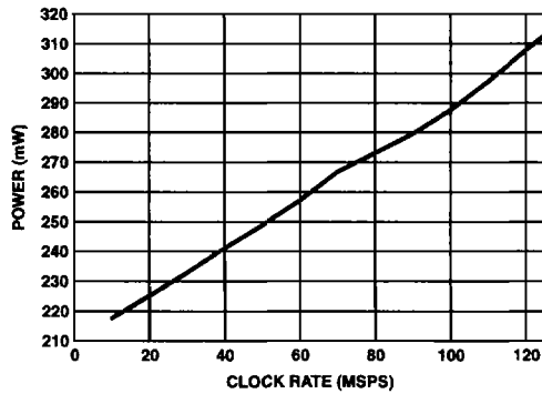
FIGURE 19. POWER vs CLOCK RATE, f_{CLK}/f_{OUT} = 10 , I_{OUT} = 20mA
