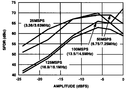
FIGURE 27. SFDR vs AMPLITUDE OF TWO TONES, f_{CLK}/f_{OUT} = 7
