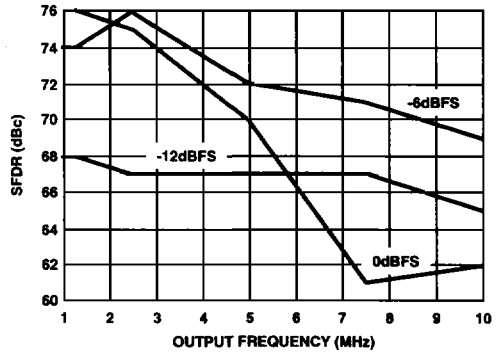
FIGURE 2. SFDR vs f_{OUT} , CLOCK = 25MSPS
