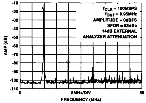
FIGURE 31. SINGLE TONE SFDR
