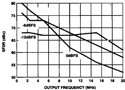
FIGURE 22. SFDR vs f_{OUT} , CLOCK = 50MSPS
