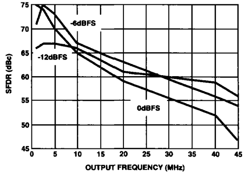
FIGURE 4. SFDR vs f_{OUT} , CLOCK = 100MSPS
