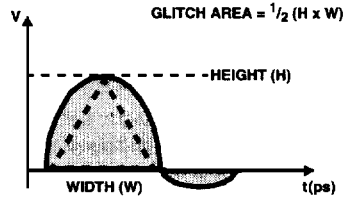
FIGURE 40. PEAK GLITCH AREA (SINGLET) MEASUREMENT METHOD
