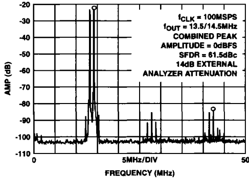
FIGURE 32. TWO-TONE, CLOCK = 100MSPS
