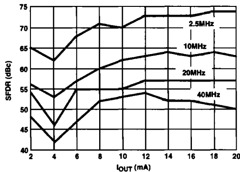
FIGURE 9. SFDR vs I_{OUT} , CLOCK = 100MSPS
