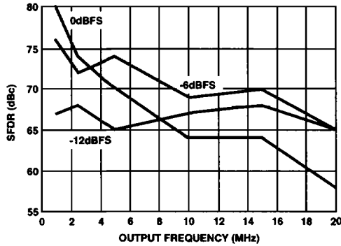
FIGURE 3. SFDR vs f_{OUT} , CLOCK = 50MSPS
