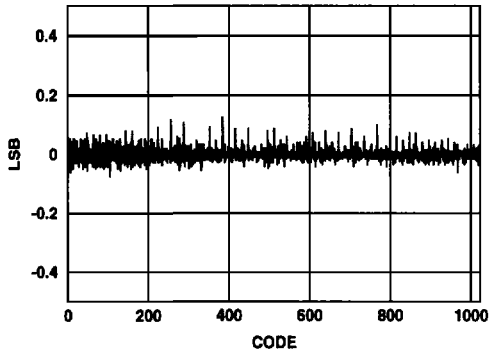
FIGURE 36. DIFFERENTIAL NONLINEARITY
