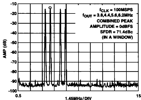
FIGURE 14. FOUR-TONE, CLOCK = 100MSPS
