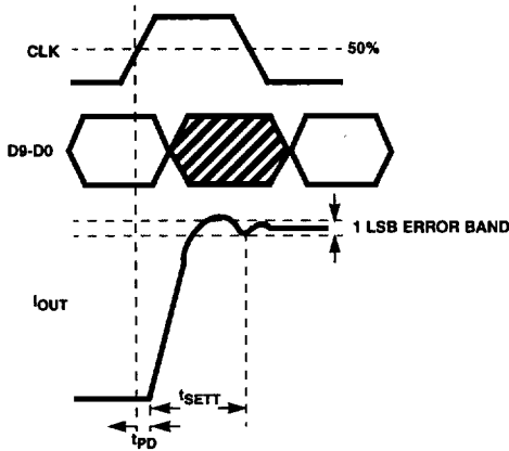
FIGURE 39. OUTPUT SETTLING TIME DIAGRAM
