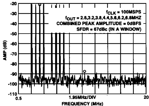
FIGURE 15. EIGHT-TONE, CLOCK = 100MSPS
