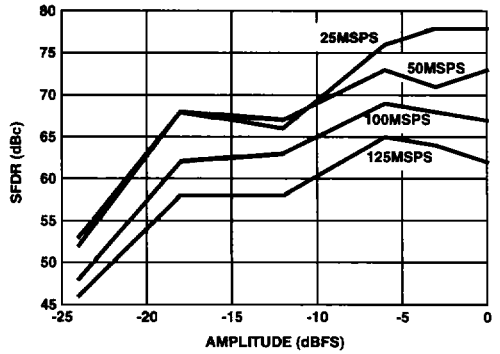
FIGURE 25. SFDR vs AMPLITUDE, f_{CLK}/f_{OUT} = 10
