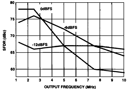
FIGURE 21. SFDR vs f_{OUT} , CLOCK = 25MSPS
