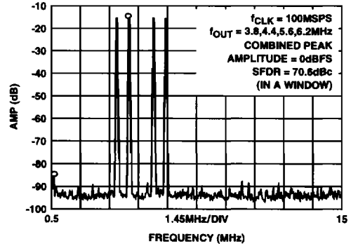
FIGURE 33. FOUR-TONE, CLOCK = 100MSPS
