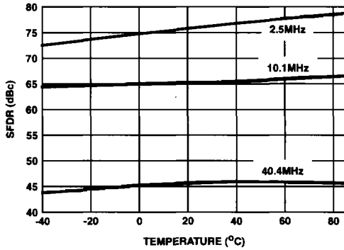
FIGURE 30. SFDR vs TEMPERATURE, CLOCK = 100MSPS
