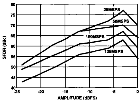
FIGURE 7. SFDR vs AMPLITUDE, f_{CLK}/f_{OUT} = 5
