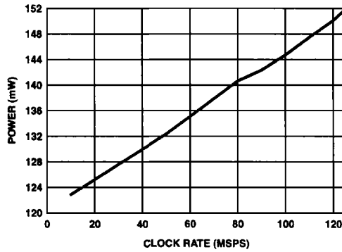
FIGURE 38. POWER vs CLOCK RATE, f_{CLK}/f_{OUT} = 10 , I_{OUT} = 20mA
