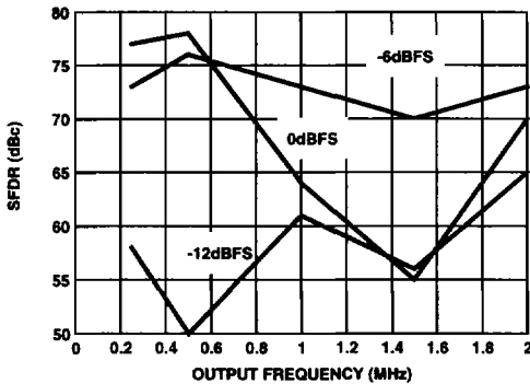
FIGURE 20. SFDR vs f_{OUT} , CLOCK = 5MSPS
