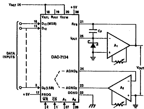
Figure 6. Unipolar Binary Operation with Forced Ground
