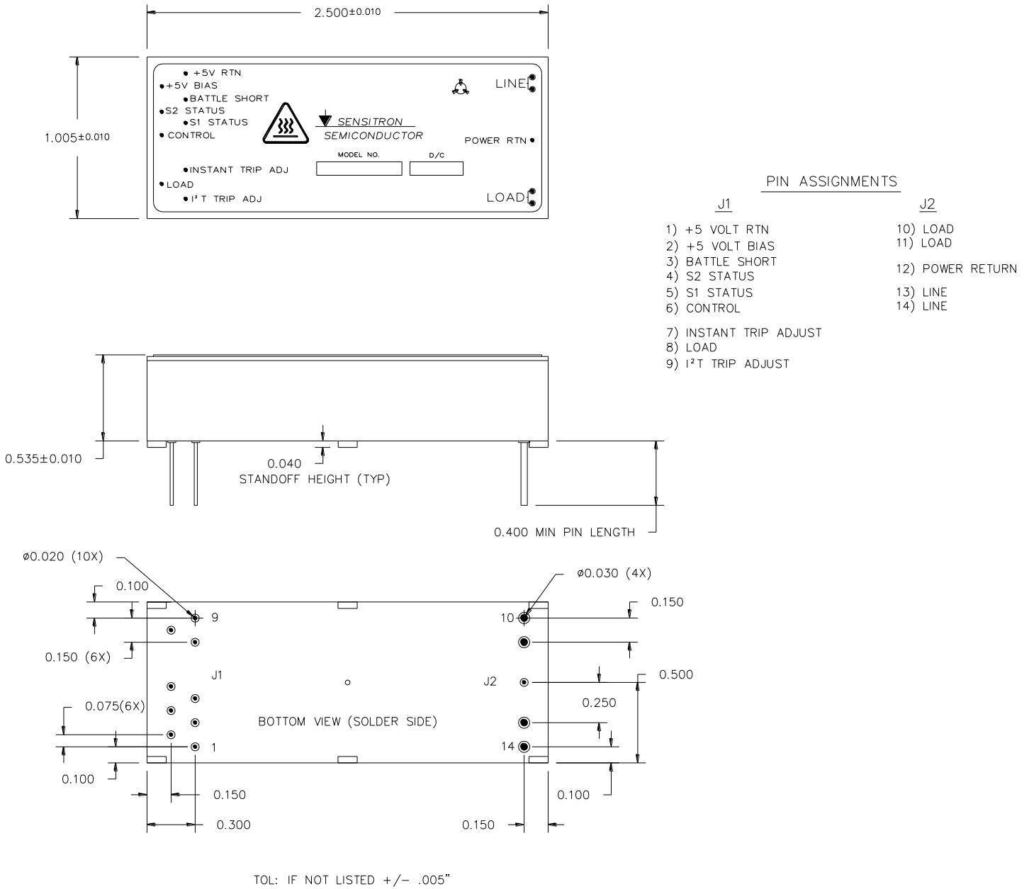
Figure 2 - Mechanical Dimensions and Pin Assignments All dimensions are in inches
