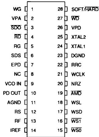
28-Pin DIP
