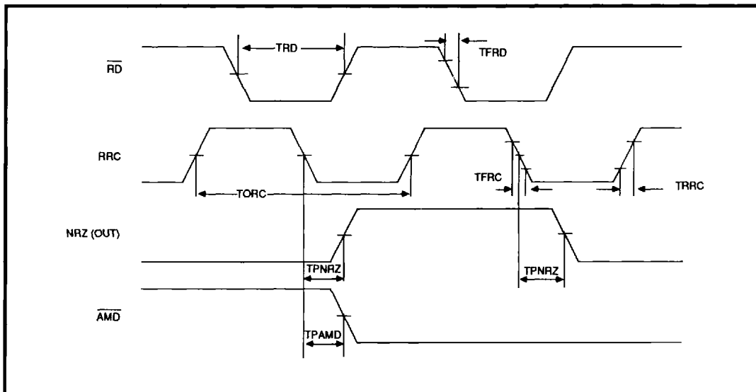
FIGURE 9: Read Timing
