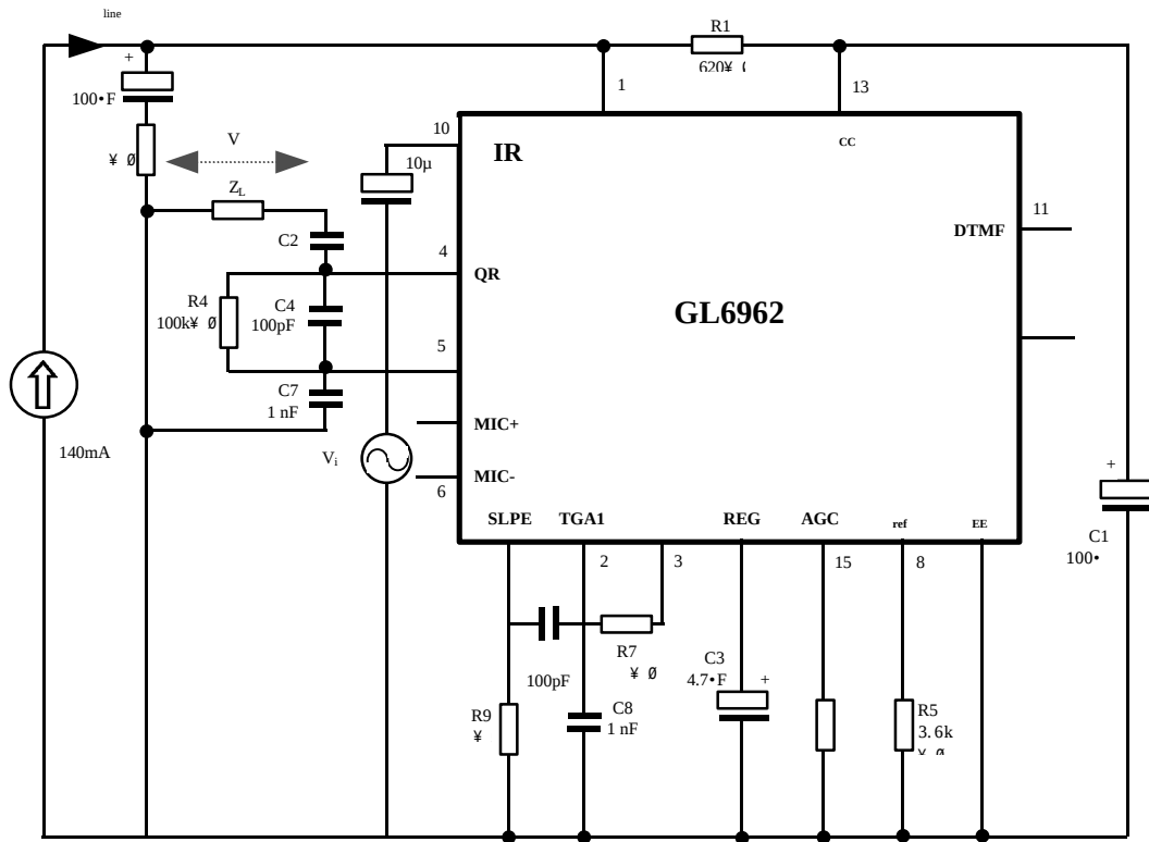
Fig. 3 Test circuit for defining GL696 (Voltage gain is defined as G = 20 \log |v_o/v_i| )
