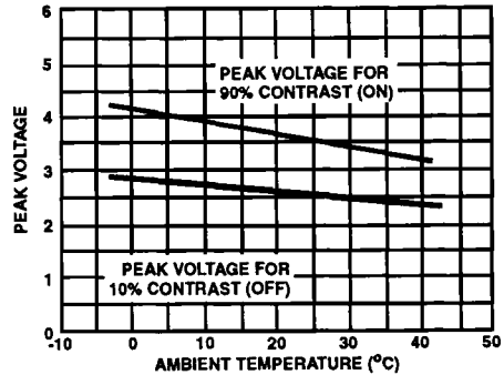
FIGURE 9. TEMPERATURE DEPENDENCE OF LC THRESHOLD
