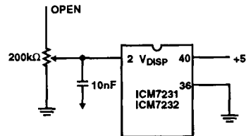
FIGURE 10. SIMPLE DISPLAY VOLTAGE ADJUSTMENT
