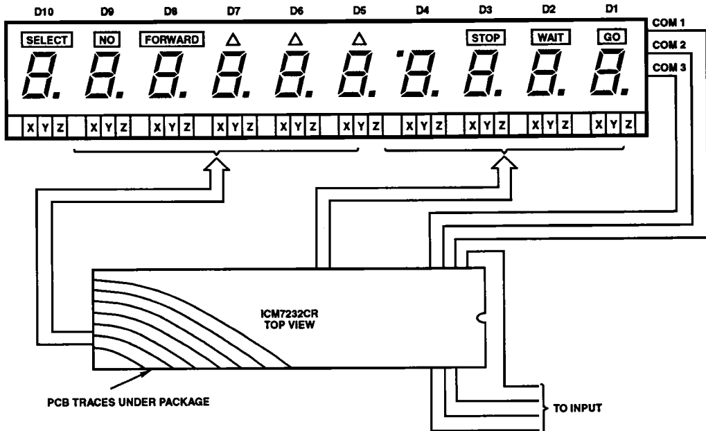
FIGURE 17. "REVERSE" PIN ORIENTATION AND DISPLAY CONNECTIONS
