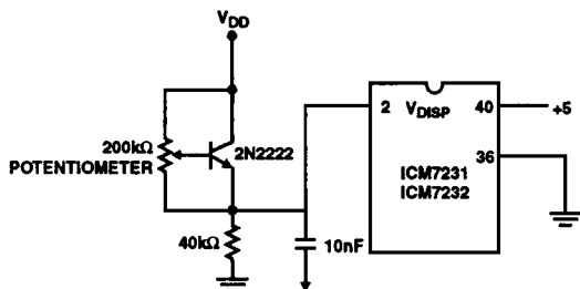
FIGURE 11B. TRANSISTOR-MULTIPLIER
