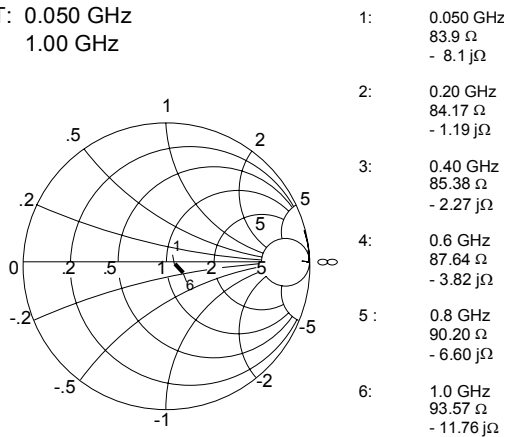
Figure 9: Output Impedance
