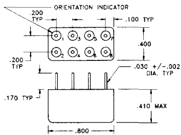
Outline 102
