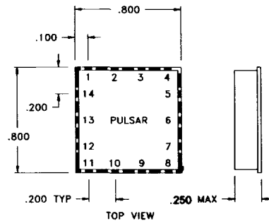
Outline F
