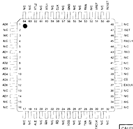
64-Lead TQFP
