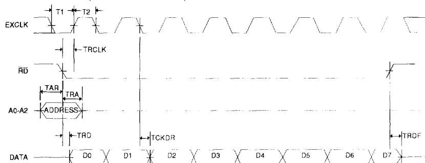
READ TIMING DIAGRAM (SERIAL VERSION)
