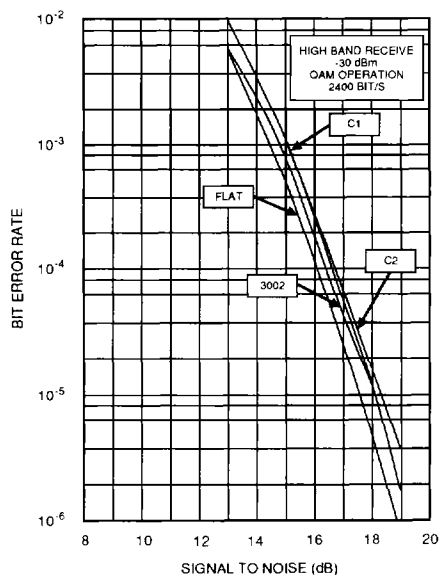
SSI 73K224L BER vs S/N-QAM-HIGH BAND
