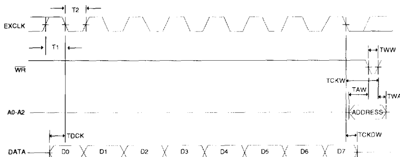
WRITE TIMING DIAGRAM (SERIAL VERSION)
