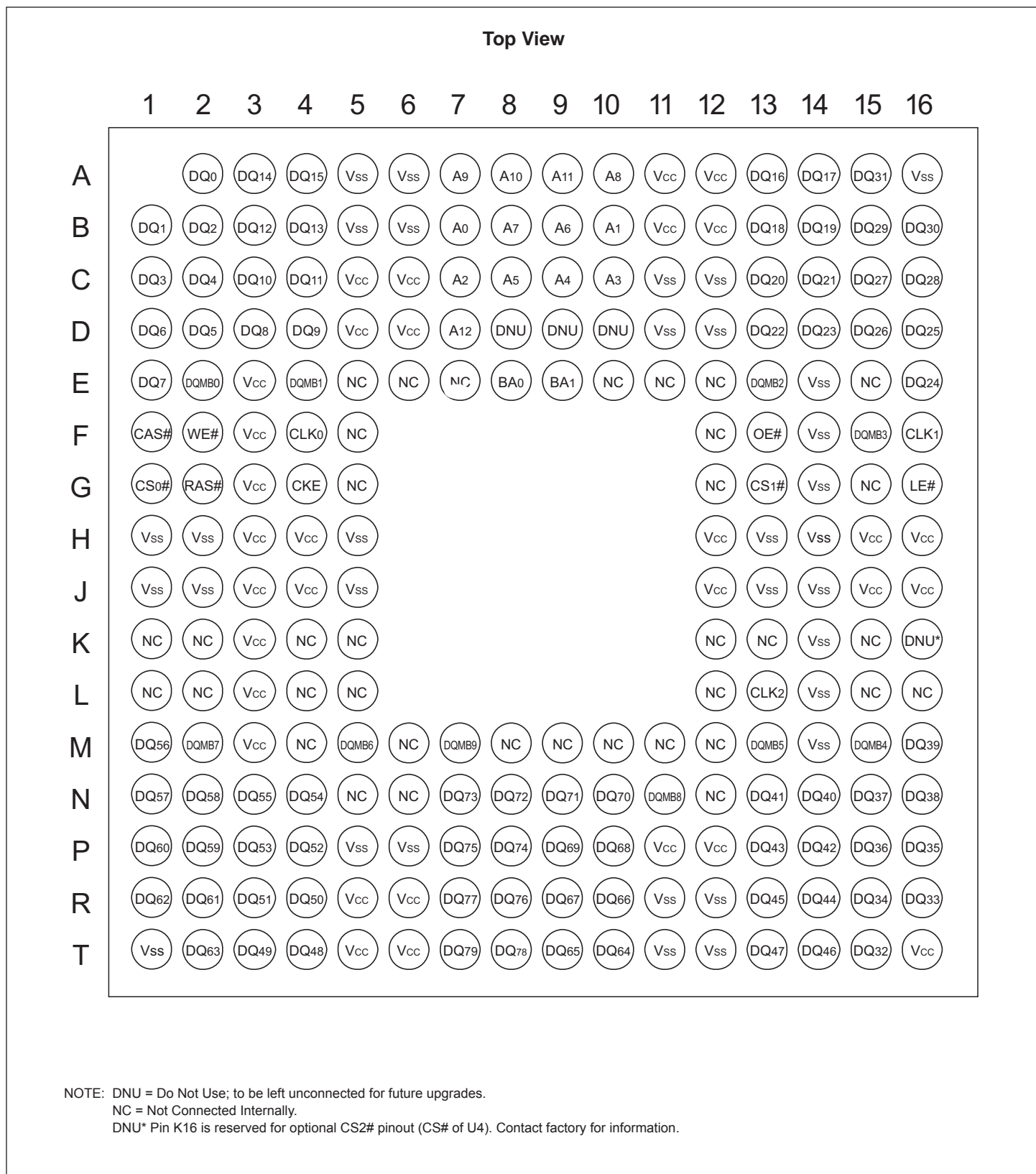
FIGURE 1 – PIN CONFIGURATION
