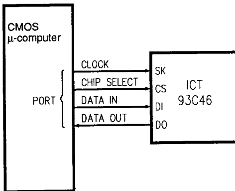
Interfacing the 93C46
