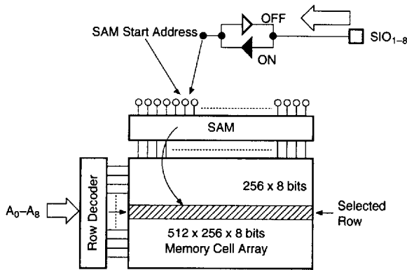
Figure 9. Block Diagram for Write Transfer Operation
