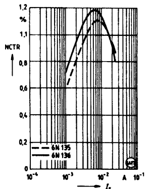
Figure 13. Current Transfer Ratio (normalized) vs. Forward Current I_F=16\text{ mA} , V_O=0.4\text{ V} , V_{CC}=5.0\text{ V} , T_A=25^\circ\text{C}
