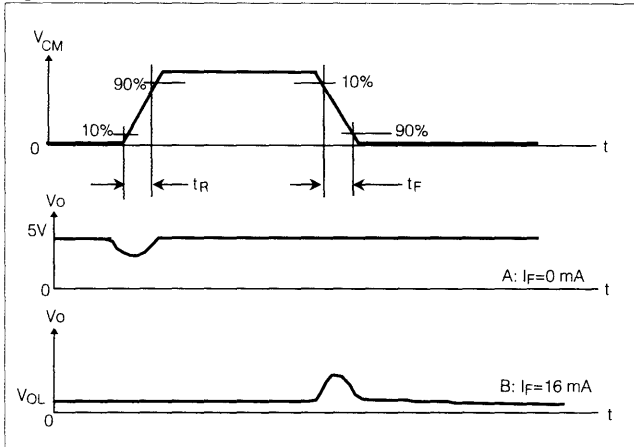
Figure 4. Measurement Waveform of CMR
