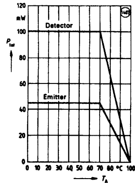
Figure 7. Permissible Total Power Dissipation vs. Ambient Temperature
