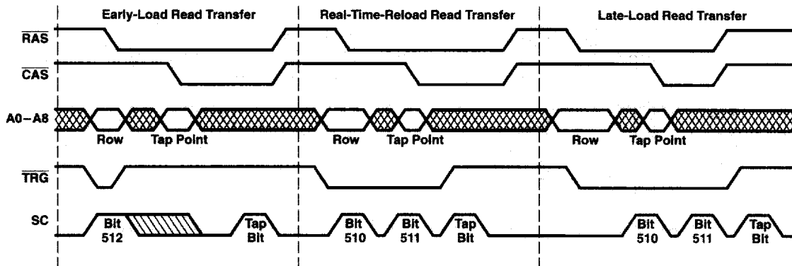
Figure 7. Normal-Read-Transfer Timings
