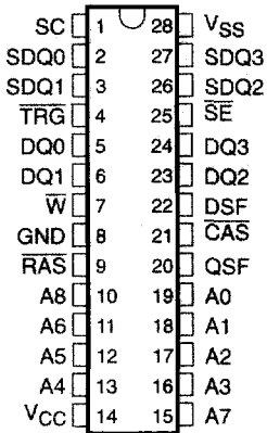
HJ PACKAGE (TOP VIEW)
