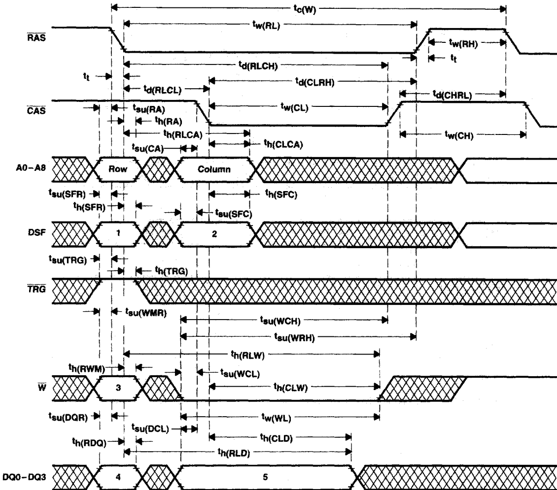
Figure 14. Early-Write-Cycle Timing
