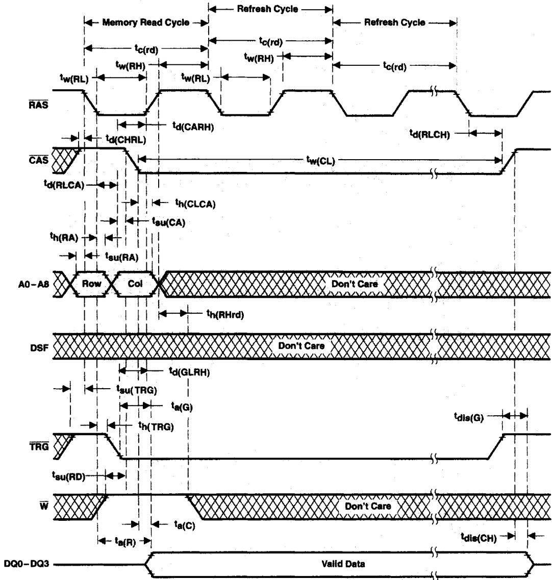
Figure 27. Hidden-Refresh-Cycle Timing
