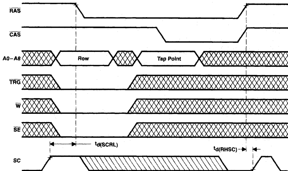
Figure 6. Normal-Write-Transfer-Cycle Timing
