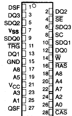
SV PACKAGE (TOP VIEW)
