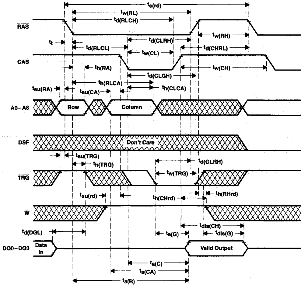
Figure 13. Read-Cycle Timing
