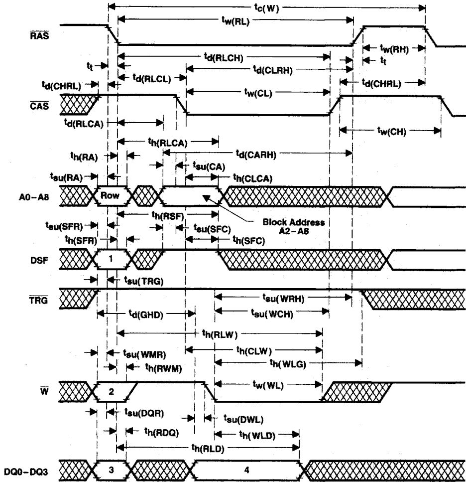
Figure 23. Block-Write-Cycle Timing (Delayed-Write)
