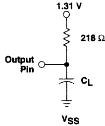
Figure 12. Load Circuit
