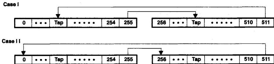
Figure 11. Serial Pointer for Split-Register Read
