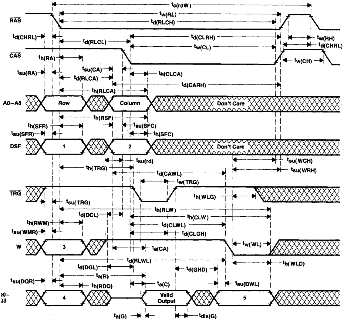
Figure 16. Read-Write/Read-Modify-Write-Cycle Timing
