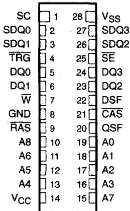
HM PACKAGE (TOP VIEW)
