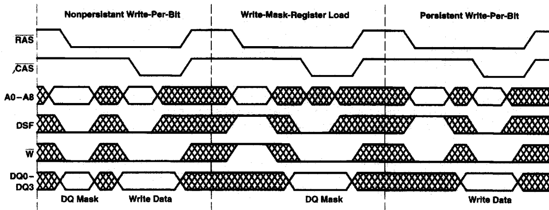
Figure 1. Example of Write-Per-Bit Operations
