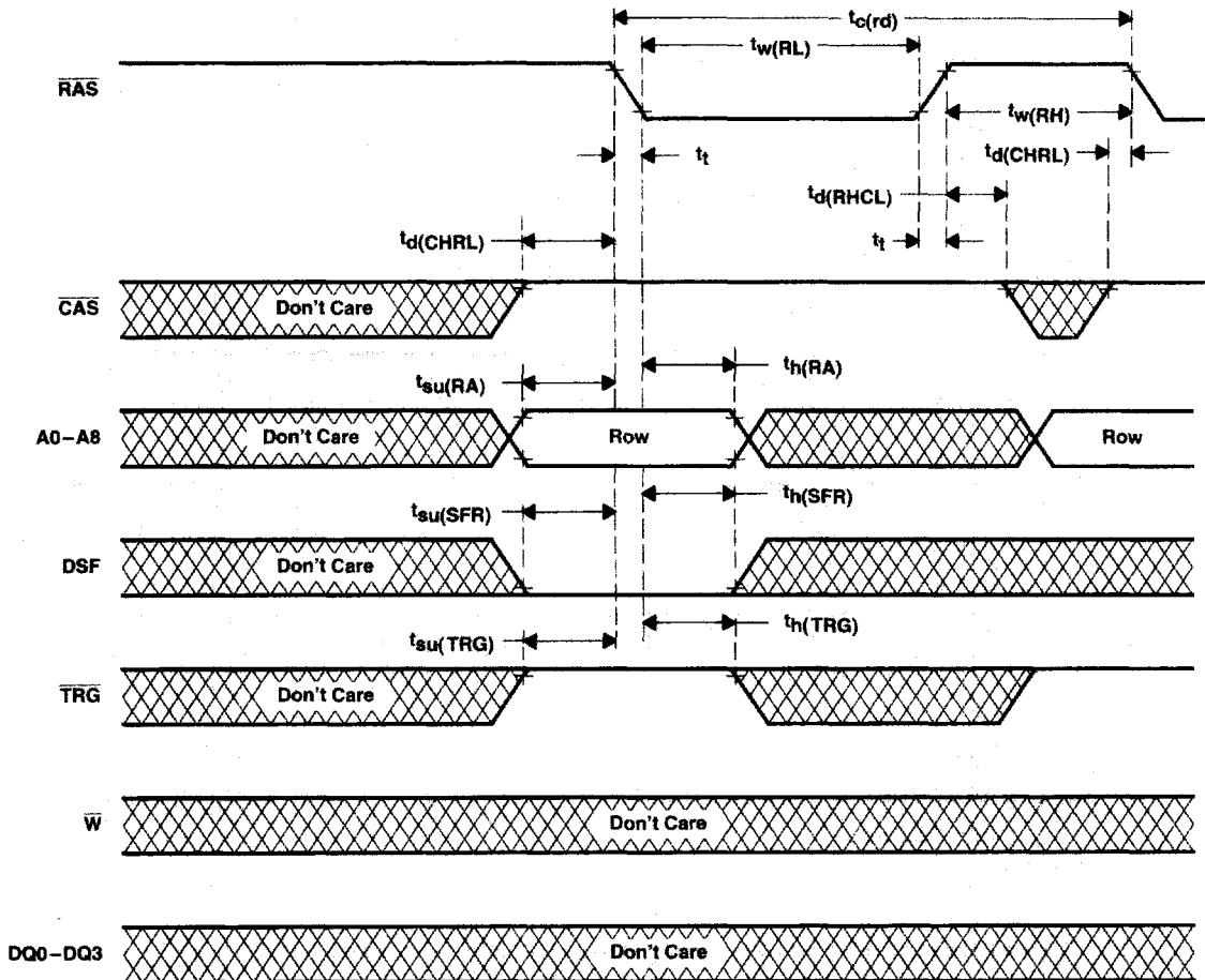
Figure 25. \overline{\text{RAS}} -Only Refresh-Cycle Timing
