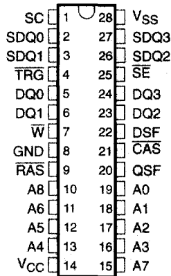
JD PACKAGE (TOP VIEW)
