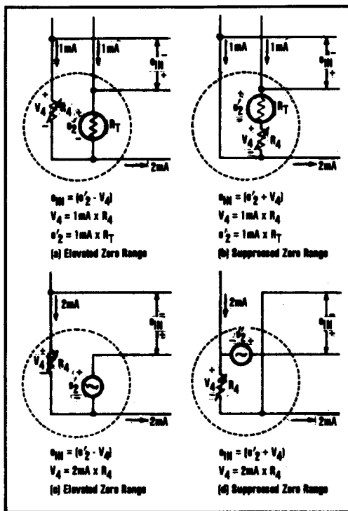
FIGURE 6. Elevation and Suppression Circuits.
