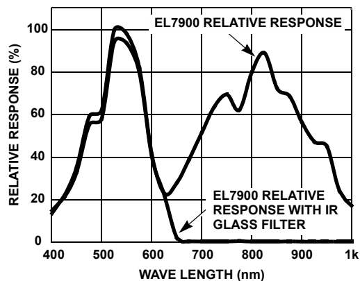
FIGURE 3. SPECTRAL RESPONSE
