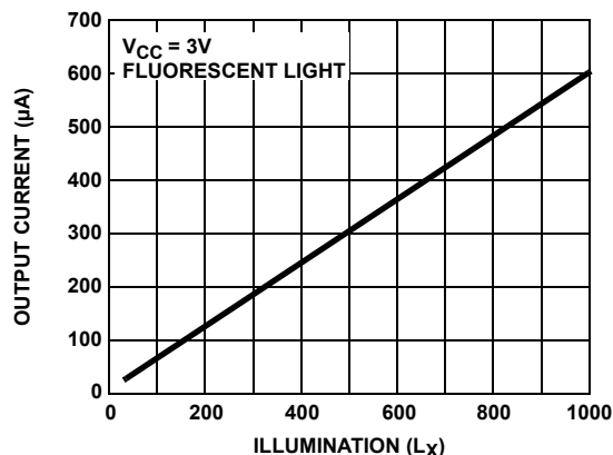
FIGURE 4. SENSITIVITY
