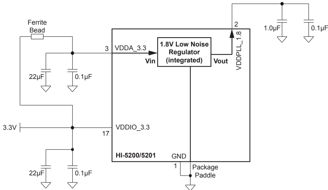
Figure 14. HI-5200/5201 Power and Ground Connections
