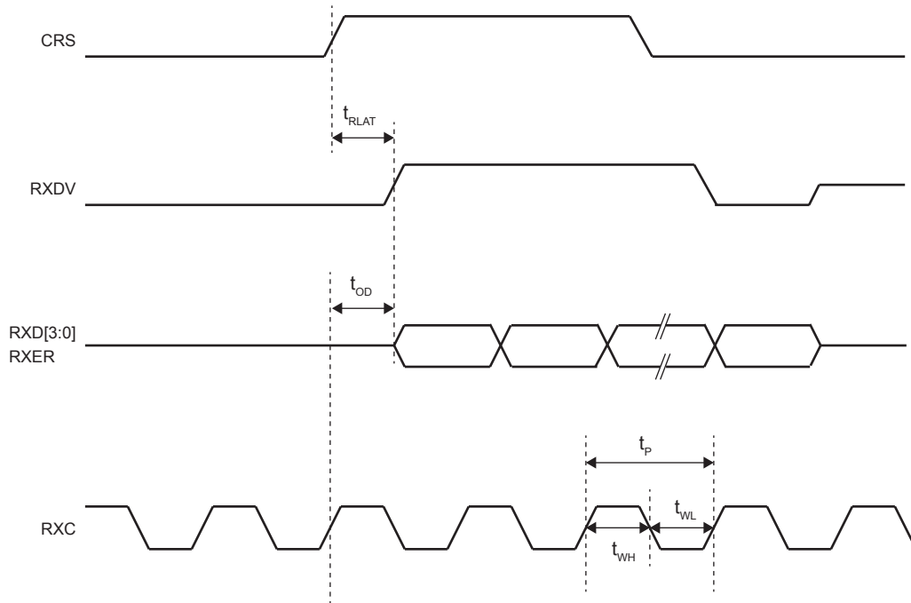
Figure 19. MII Receive Timing (100Base-Tx)
