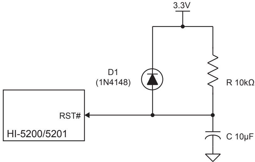
Figure 25. Recommended Reset Circuit
