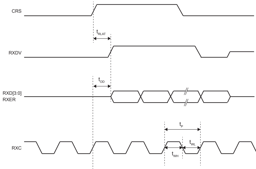
Figure 17. MII Receive Timing (10Base-T)
