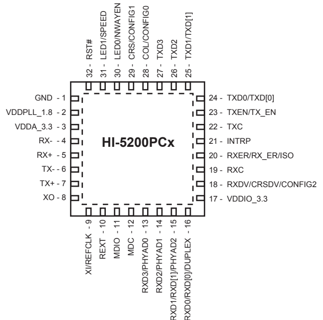
Figure 1. HI-5200: 32-Pin Plastic 5mm x 5mm QFN
