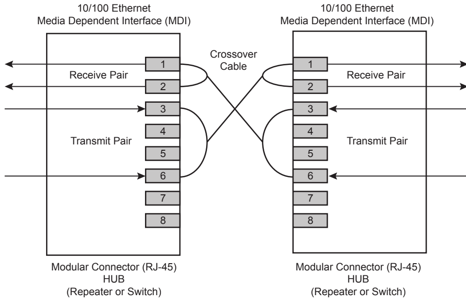
Figure 11. Typical Crossover Cable Connection
