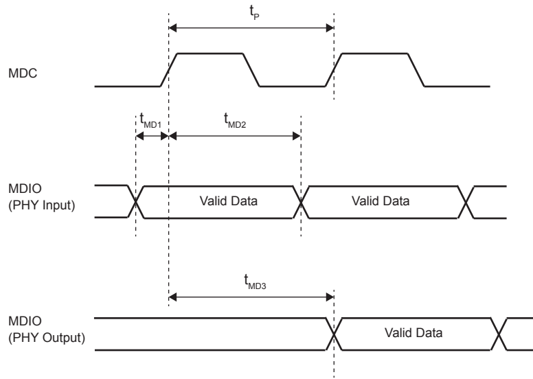
Figure 23. MDC/MDIO Timing
