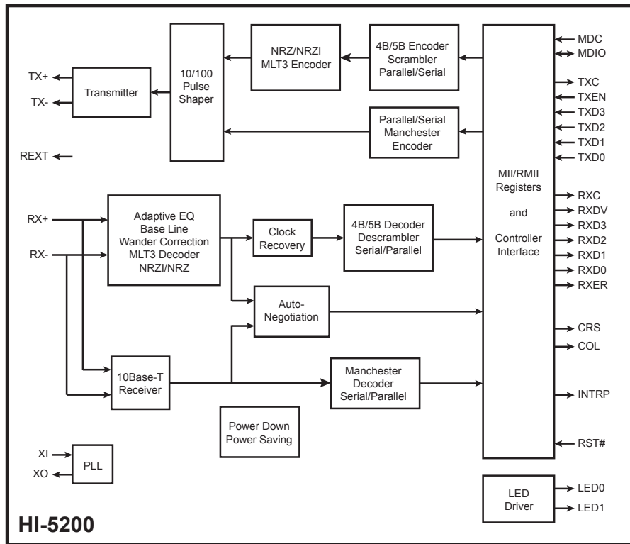
Figure 2. HI-5200 Block Diagram
