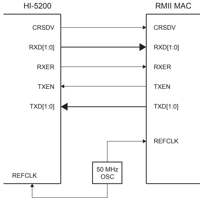
Figure 8. HI-5200 RMII Interface
