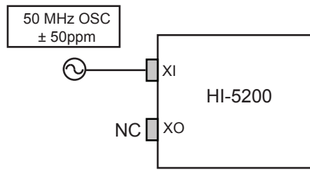
Figure 13. 50MHz Oscillator Reference Clock for HI-5200 RMII Mode
