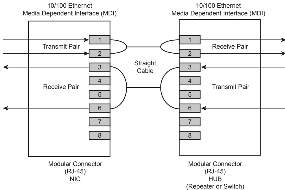
Figure 10. Typical Straight Cable Connection
