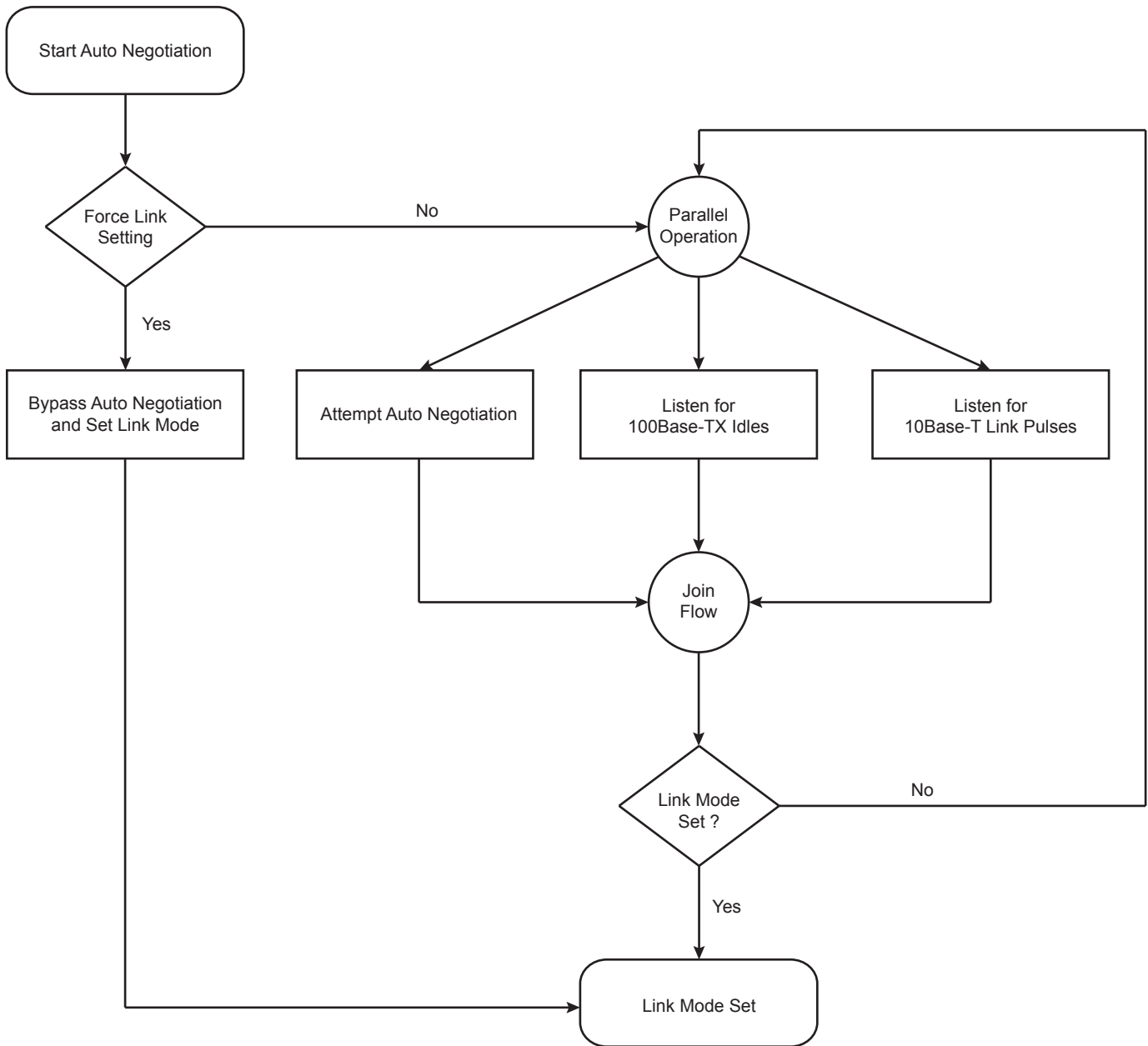
Figure 7. Auto Negotiation Flow Chart
