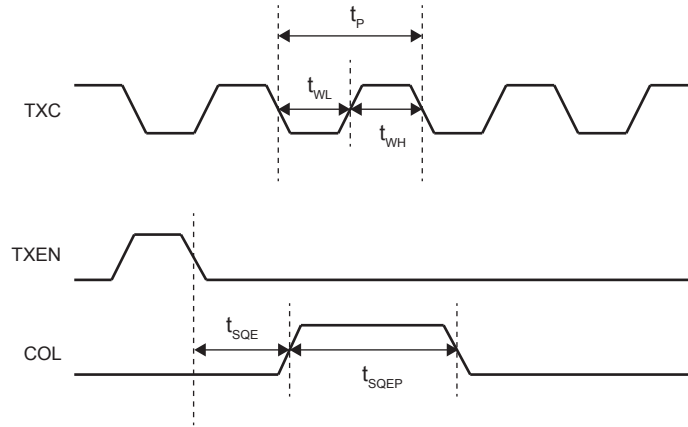
Figure 15. MII SQE Timing (10Base-T)
