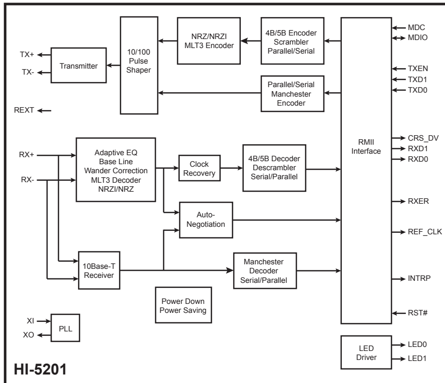
Figure 3. HI-5201 Block Diagram
