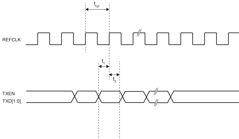
Figure 20. RMII Transmit Timing
