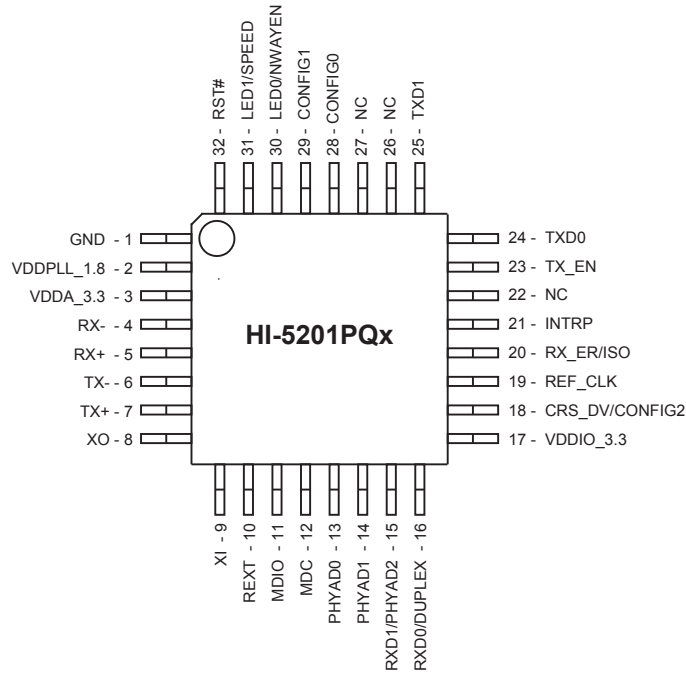
Figure 5. HI-5201: 32-Pin Plastic 9mm x 9mm TQFP
