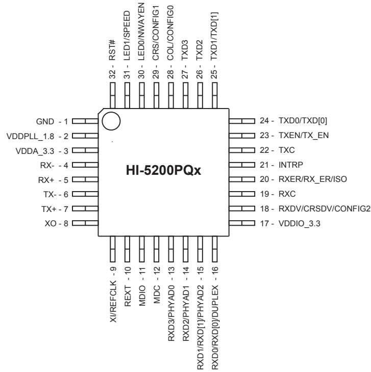
Figure 4. HI-5200: 32-Pin Plastic 9mm x 9mm TQFP
