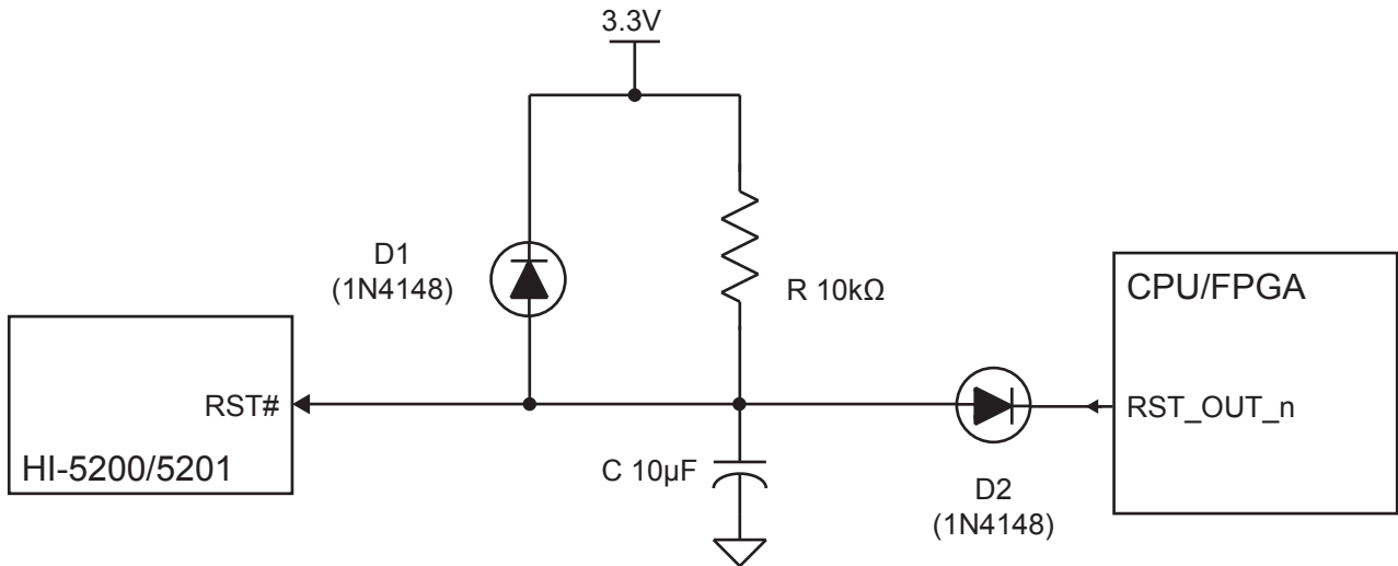
Figure 26. Recommended Reset Circuit for interfacing with CPU/FPGA Reset Output
