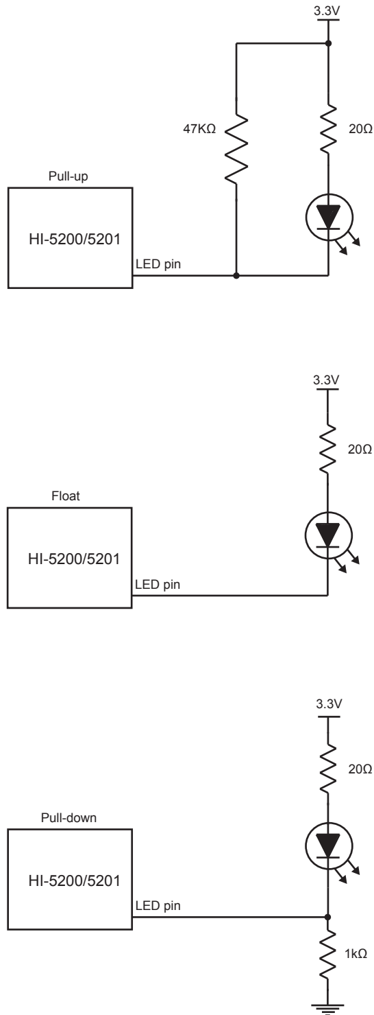
Figure 27. Reference Circuits for LED Strapping Pins
