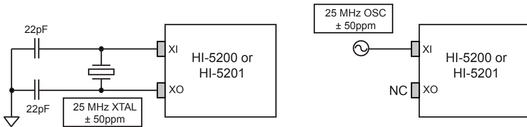
Figure 12. 25MHz Crystal/Oscillator Reference Clock for HI-5200/5201
