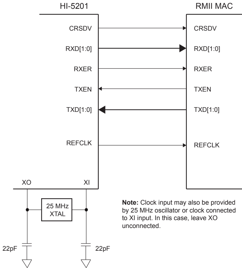
Figure 9. HI-5201 RMII Interface
