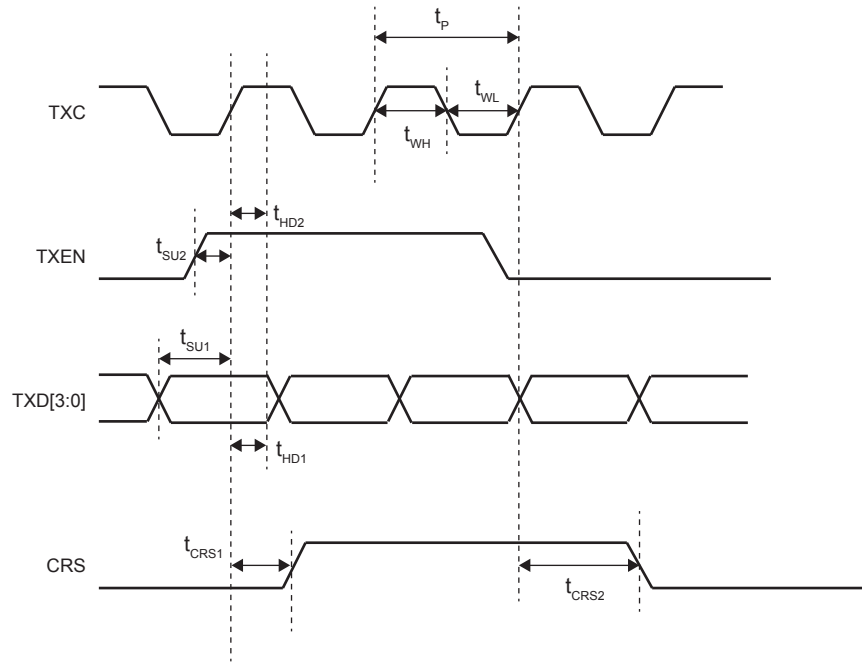
Figure 16. MII Transmit Timing (10Base-T)
