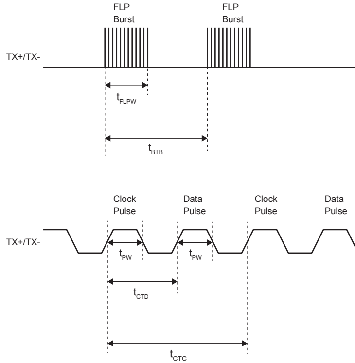
Figure 22. Auto-Negotiation Fast Link Pulse (FLP) Timing
