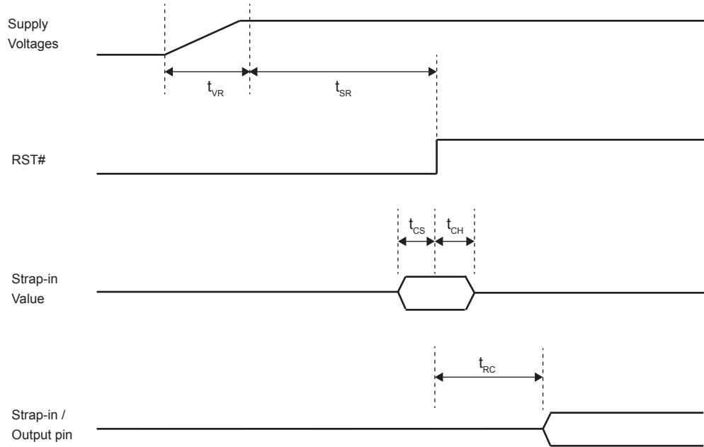
Figure 24. Power-Up/Reset Timing
