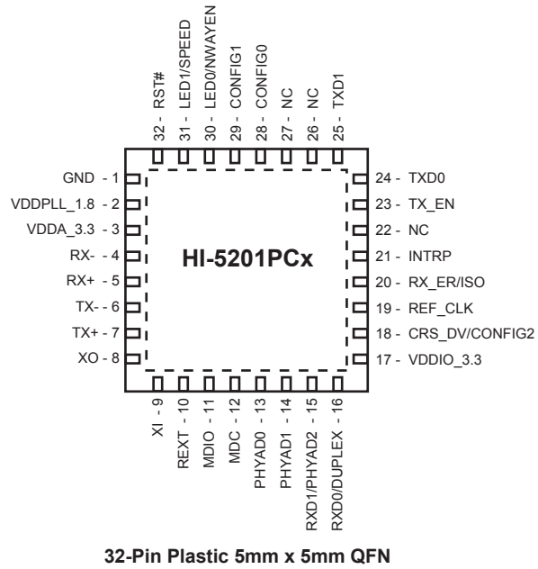
Figure 6. HI-5201: 32-Pin Plastic 5mm x 5mm QFN
