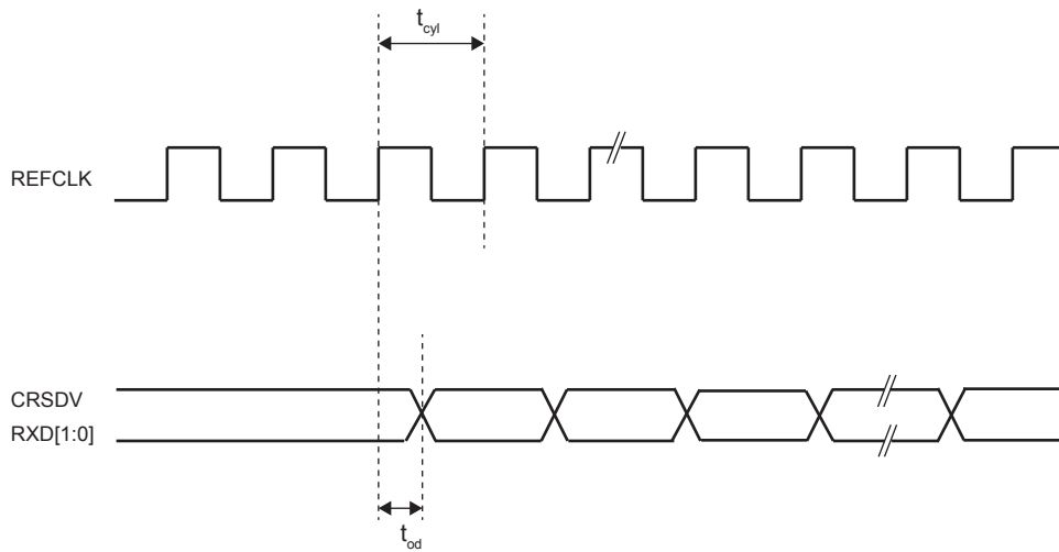
Figure 21. RMII Receive Timing
