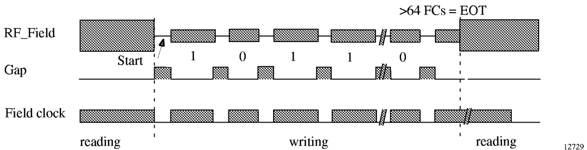
Figure 15. Signals to the transponder during writing
