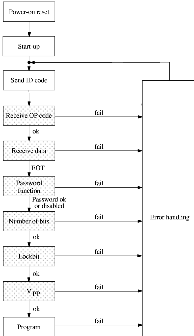
Figure 32. Simplified error handling of the e5561
