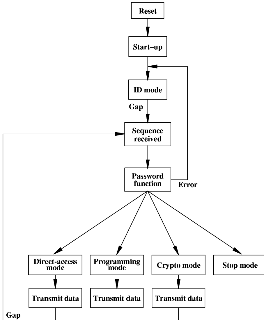
Figure 3. State diagram of the e5561 (overview)
