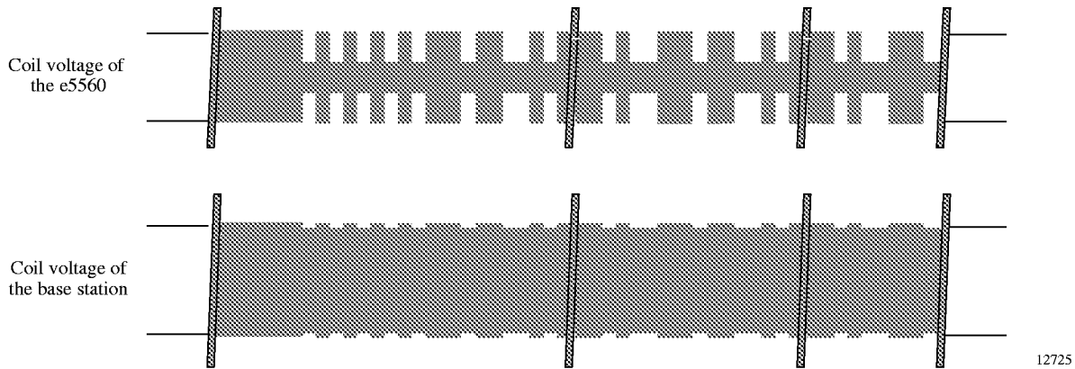
Figure 11. Signals from the transponder during reading
