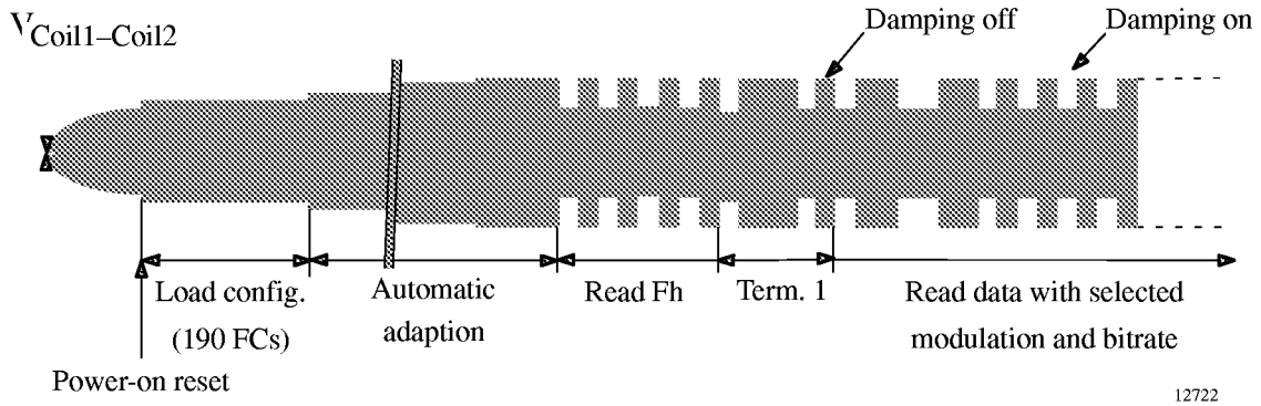
Figure 8. Voltage at Coil1/Coil2 after start-up (e.g., RF/32, Manchester, Terminator 1)
