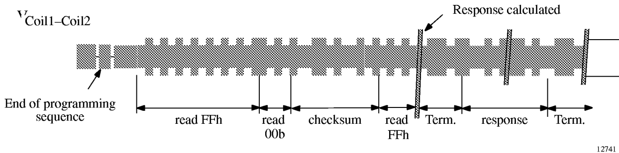
Figure 29. Coil voltage in crypto mode
