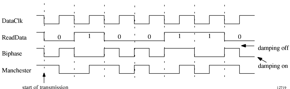
Figure 5. Types of modulation
