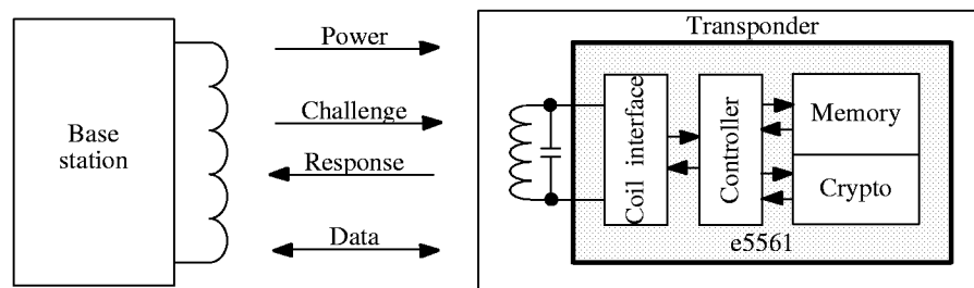
Figure 1. Transponder system example using e5561
