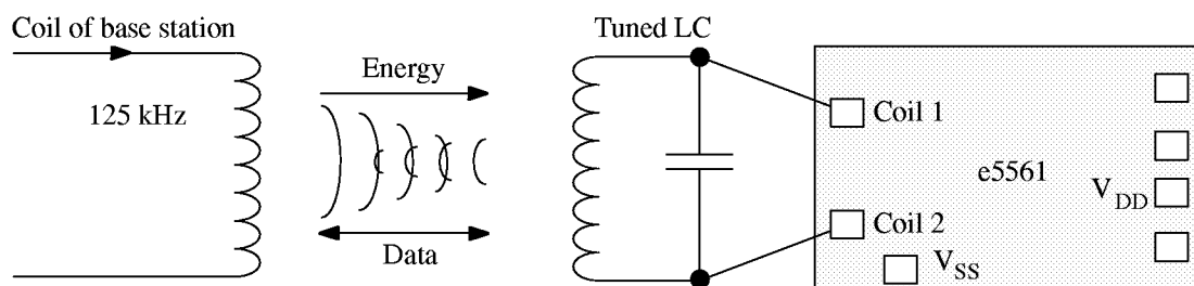
Figure 7. Application circuit
