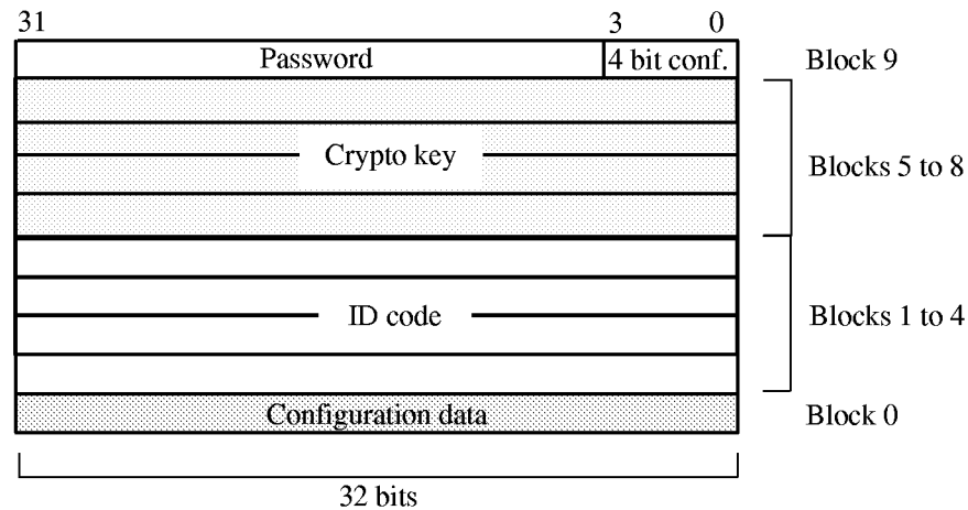
Figure 6. Memory map
