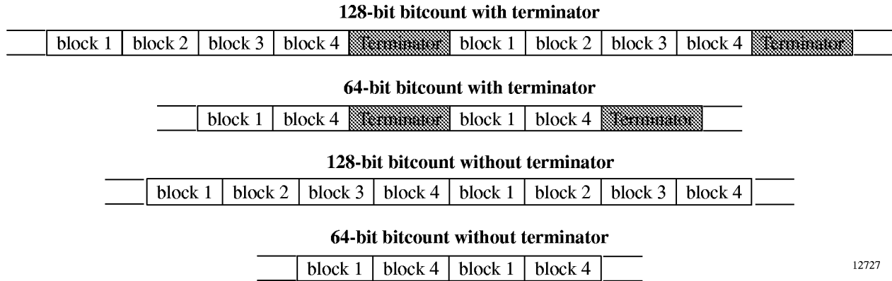
Figure 13. ID mode data streams
