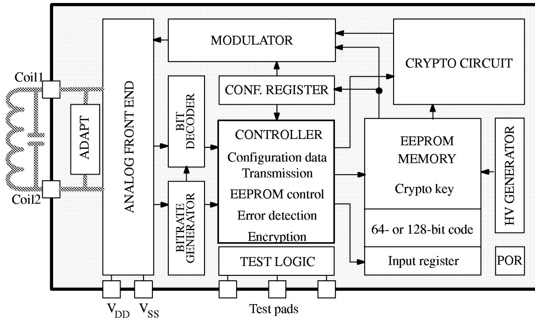
Figure 4. Block diagram
