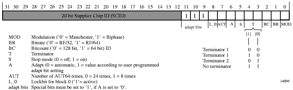
Figure 9. Configuration data in block 0
