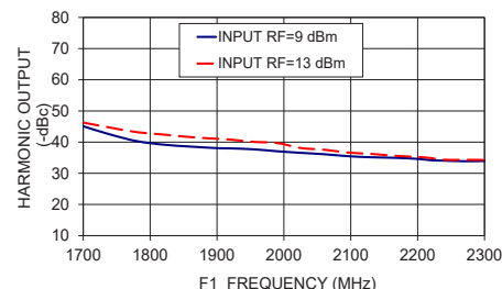
ZX90-3-692-S+ HARMONIC OUTPUT F4
