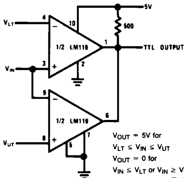
Window Detector
