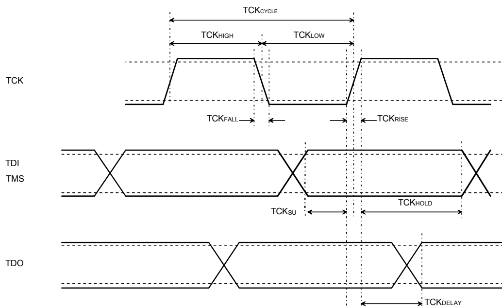
Figure 28. JTAG Timing
