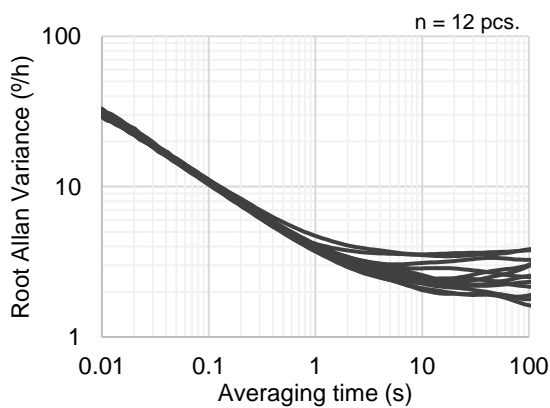
Figure. Allan Variance
