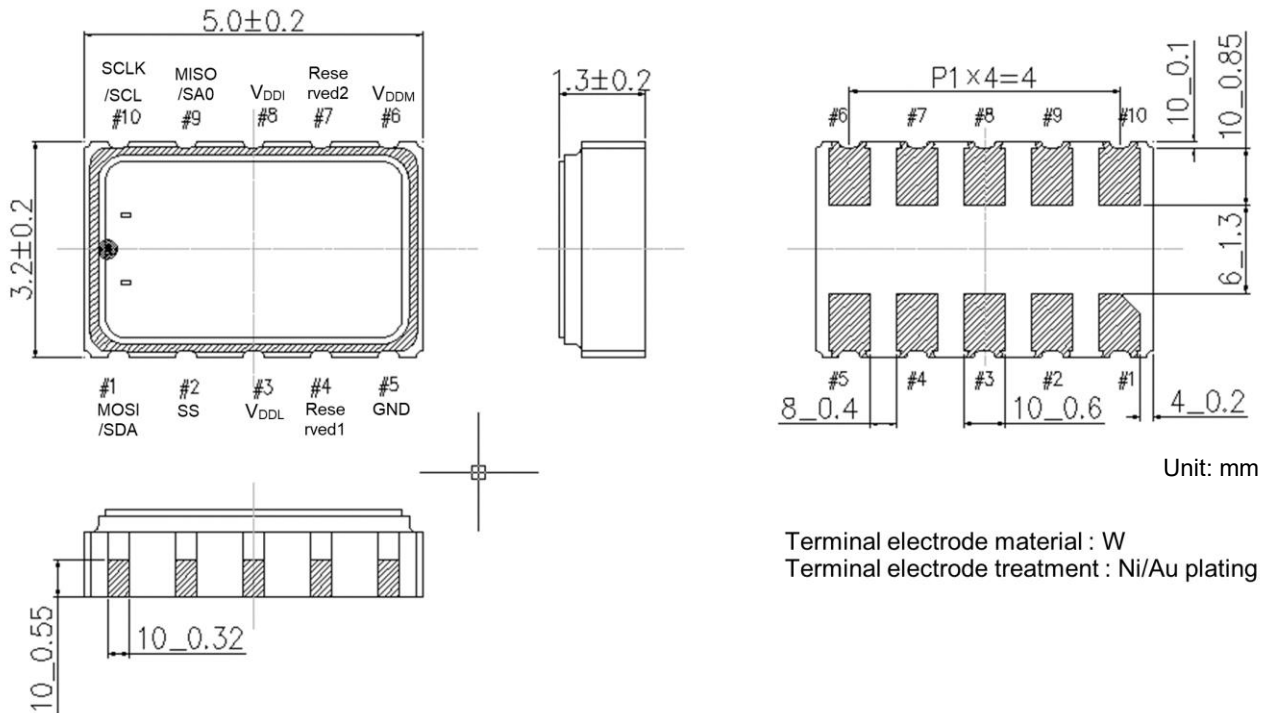
Figure 4.1. Outline Dimensions
