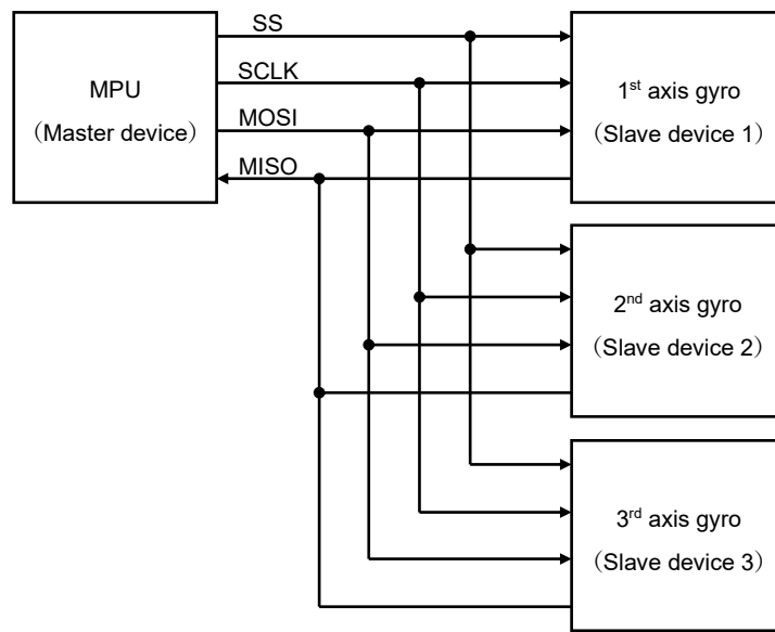
Figure 6.18. Connection Examples
