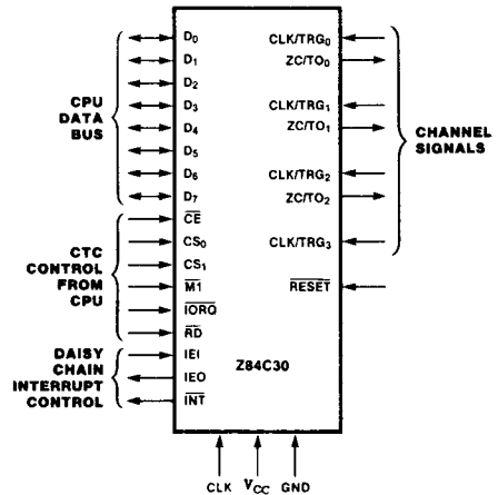
Figure 1. Logic Functions
