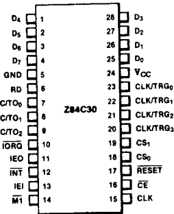
Figure 2. Pin Configuration
