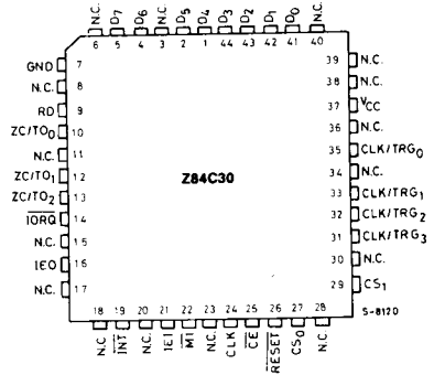
Figure 2a. Chip-Carrier Pin Configuration
