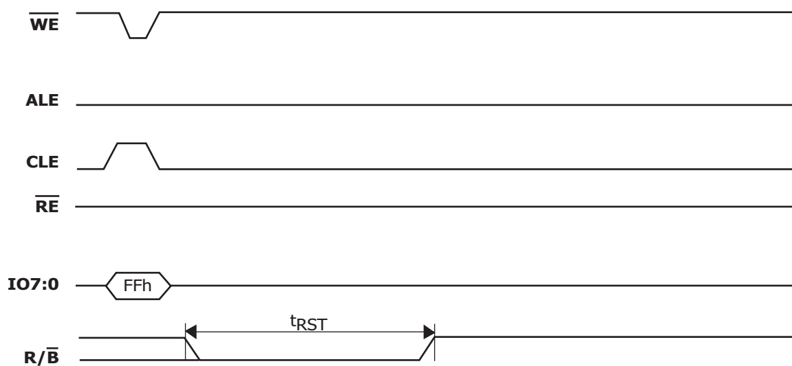
Figure 19 : Reset Operation
