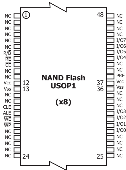
Figure 3. 48USOP1 Contactions, x8 Device
