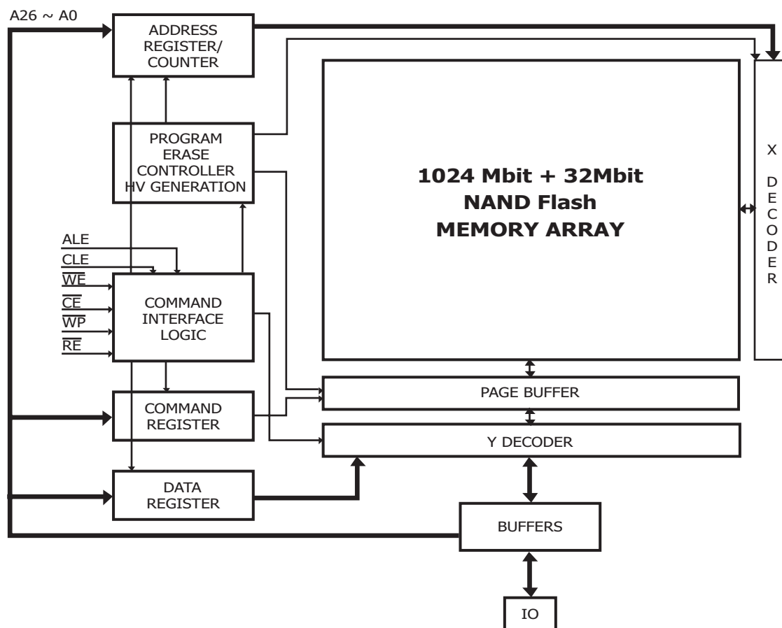
Figure 4: Block Diagram
