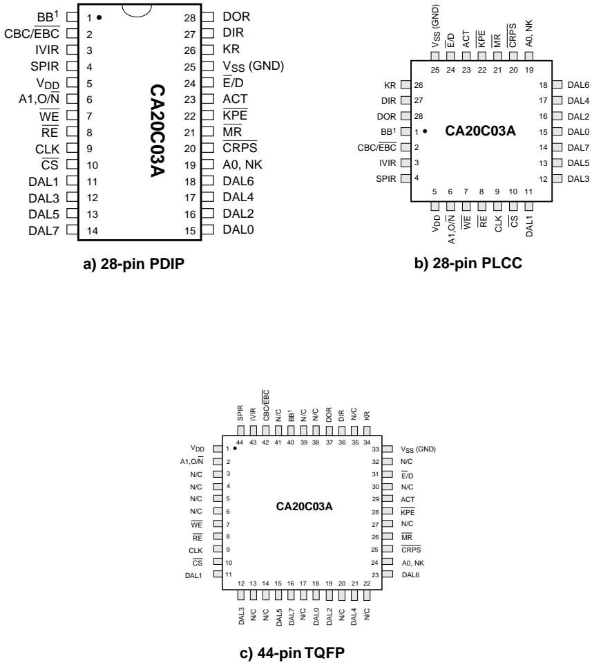
Figure 3-2 : CA20C03A Pin Configuration
