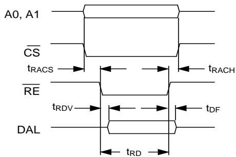
Figure 3-5 : Read Timing
