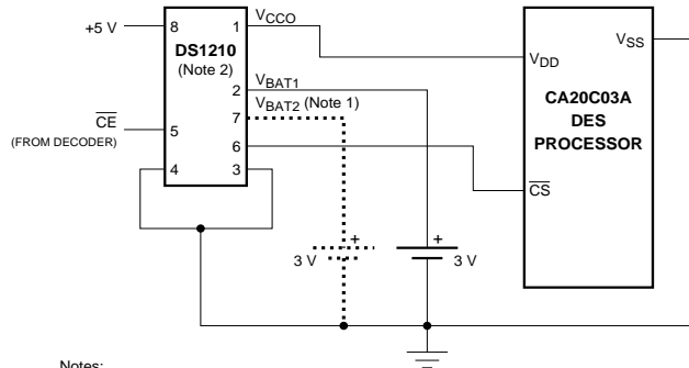
Figure 3-14 : CA20C03A Battery Back-up Circuit Example
