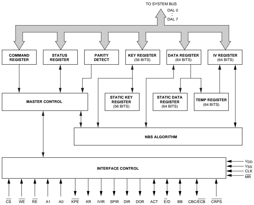
Figure 3-1 : CA20C03A Block Diagram
