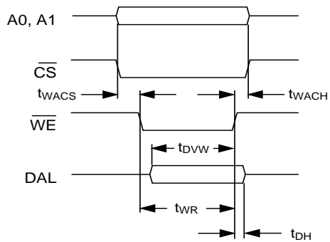
Figure 3-6 : Write Timing
