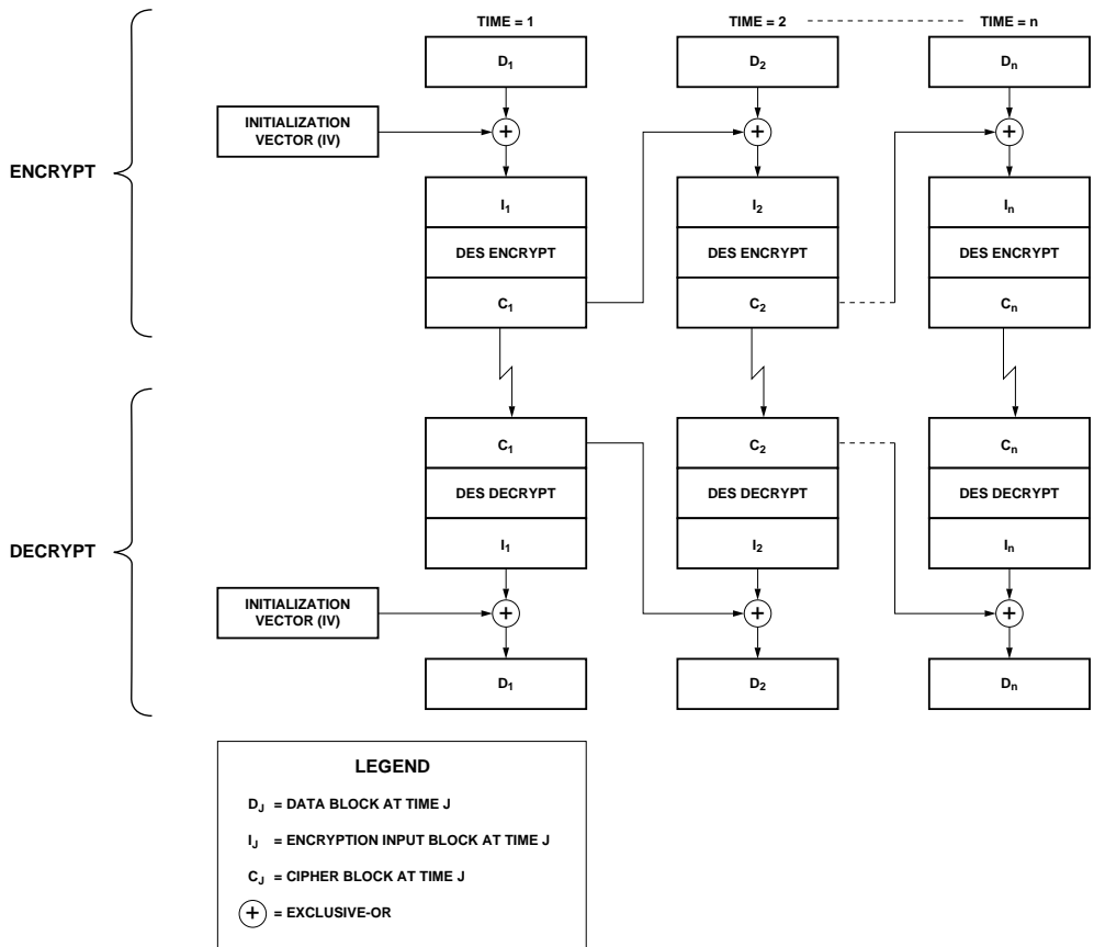
Figure 3-10 : Cipher Block Chaining (CBC) Mode
