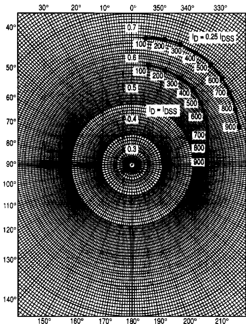
Figure 18. S 11g
