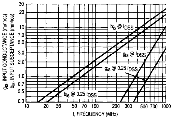
Figure 6. Input Admittance ( y_{is} )
