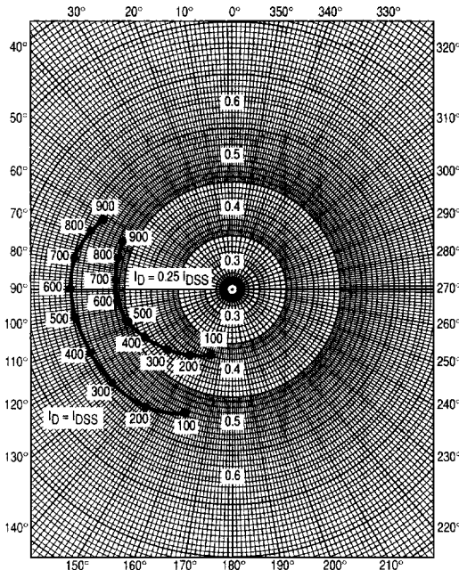
Figure 12. S_{21s}
