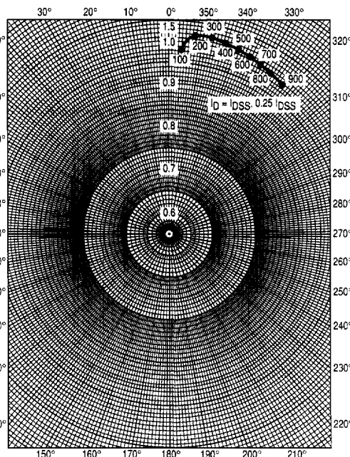
Figure 21. S 22g
