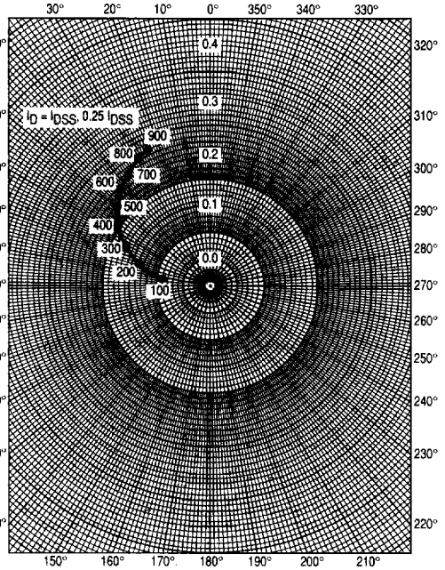
Figure 11. S_{12s}
