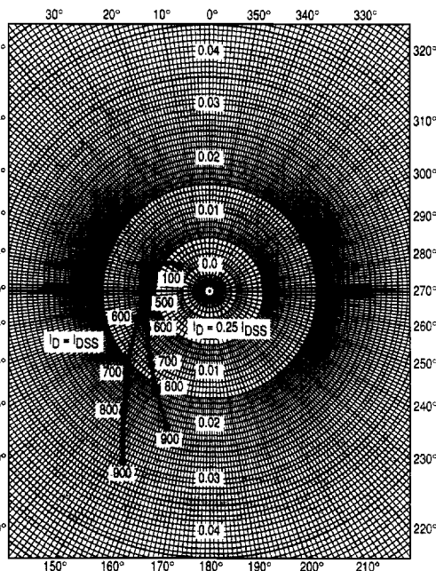
Figure 19. S 12g
