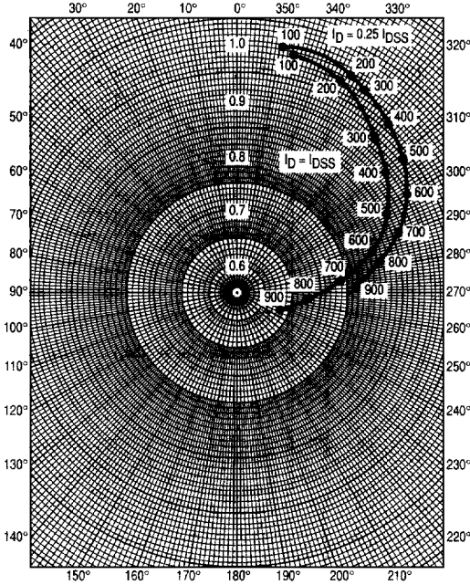
Figure 10. S_{11s}
