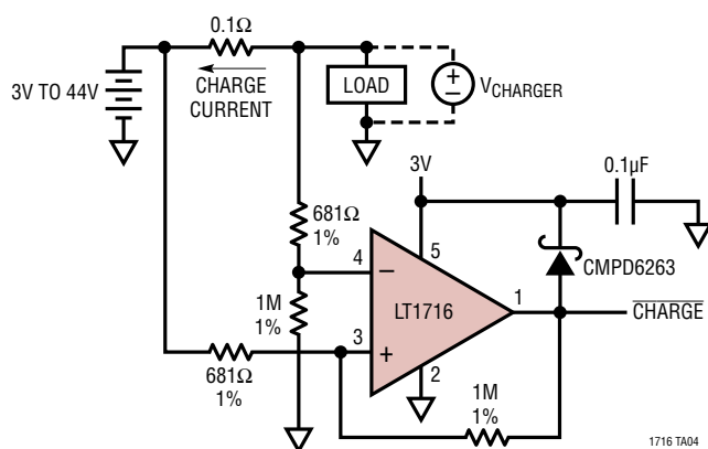
Charge/Discharge Indicator
