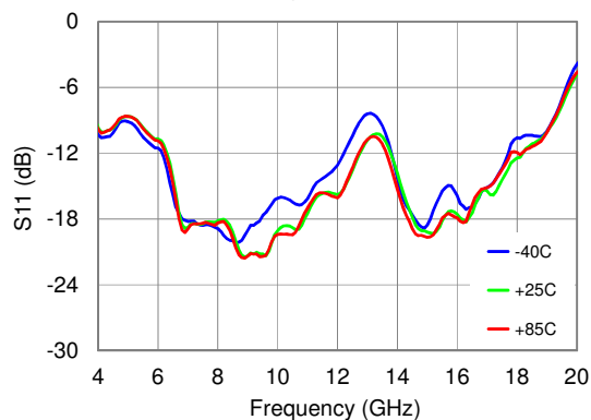
Average IRL vs. Temperature
