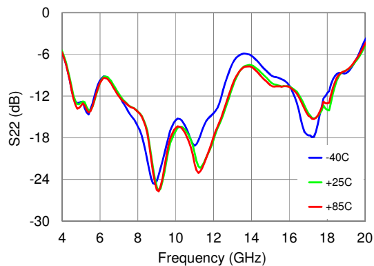
Average ORL vs. Temperature
