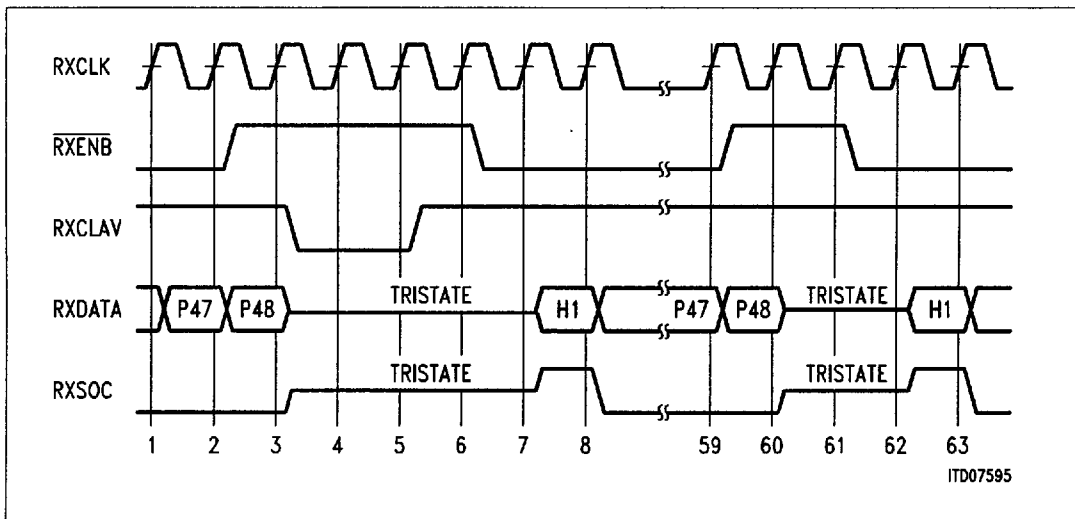
Figure 20 RxClav Example #1
