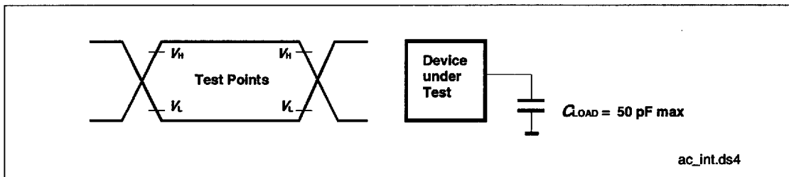
Figure 29 Input/Output waveform for AC measurements
