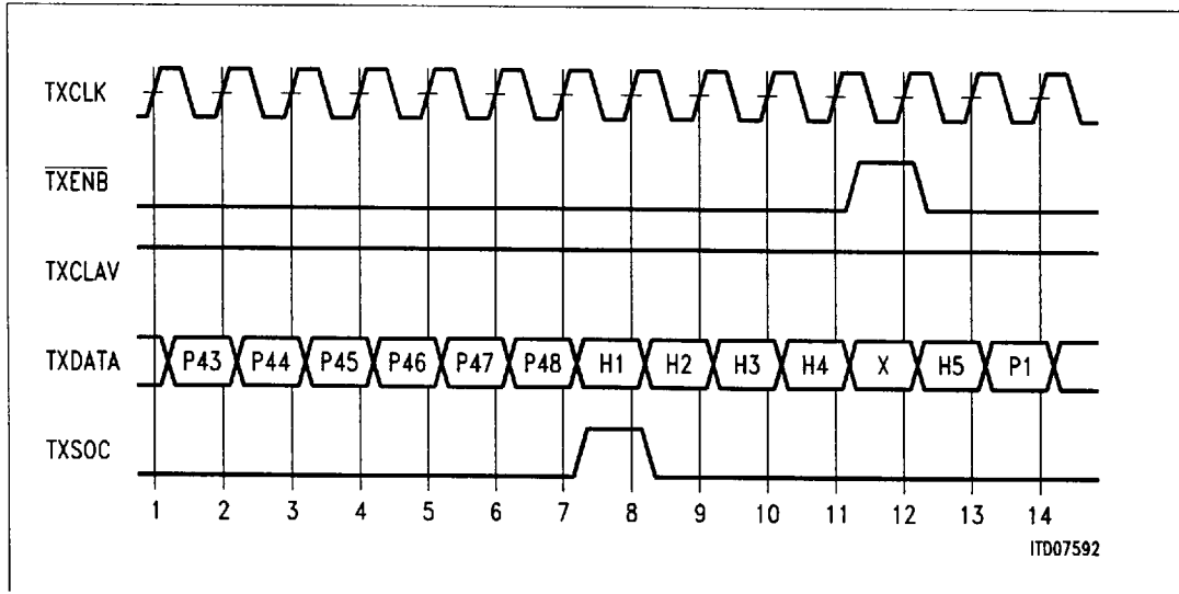
Figure 17 TxClav Example #2
