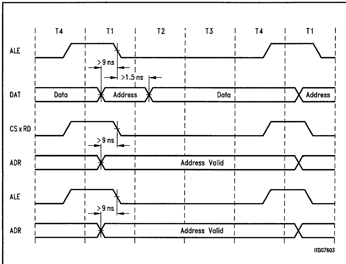
Figure 33 SDHT Address Setup and Hold Times
