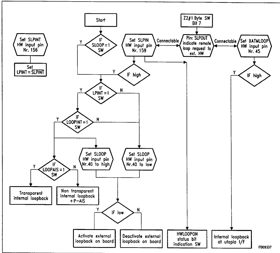
Figure 24 SDH Flow Chart for Loopback Applications
