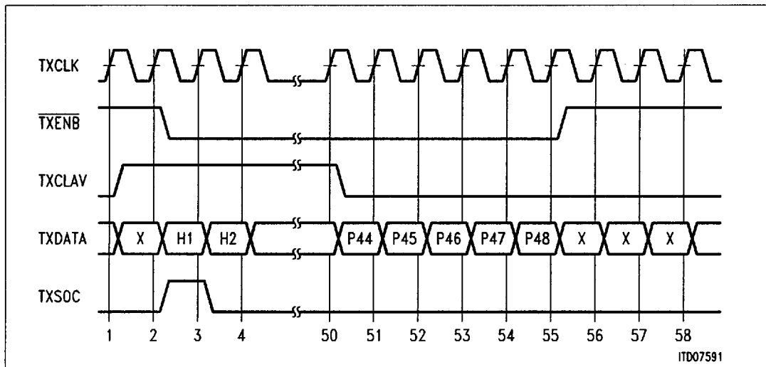
Figure 16 TxClav Example #1
