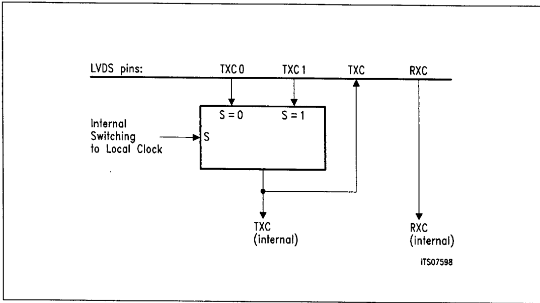
Figure 23 SDH Clock Switching
