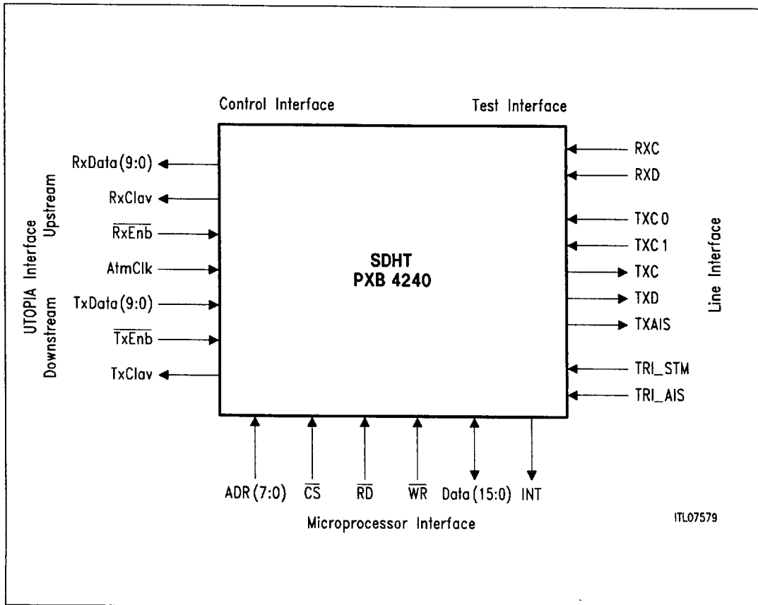
Figure 1 SDHT Logic Symbol
