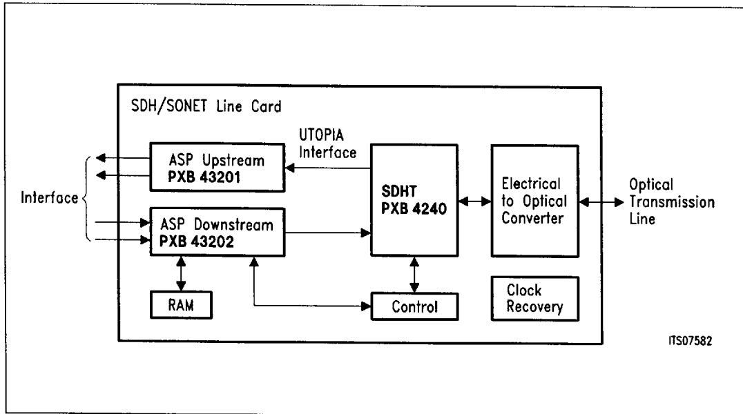
Figure 4 SDH/SONET Line Card Example
