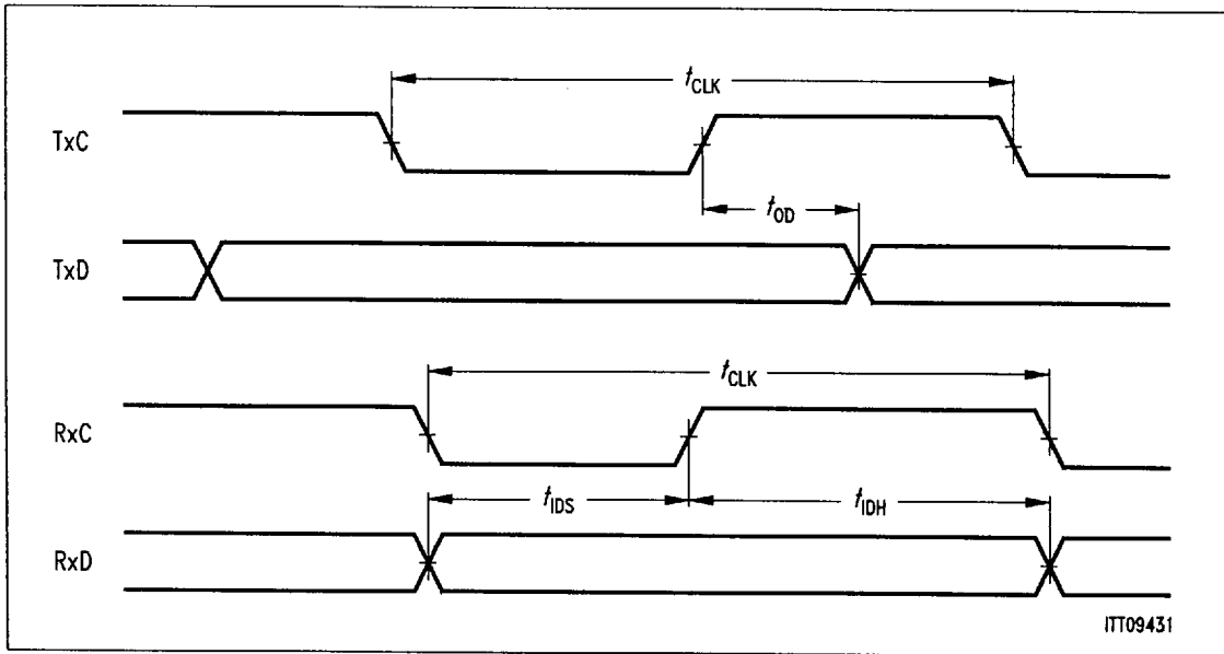
Figure 30 Line interface timing diagram
