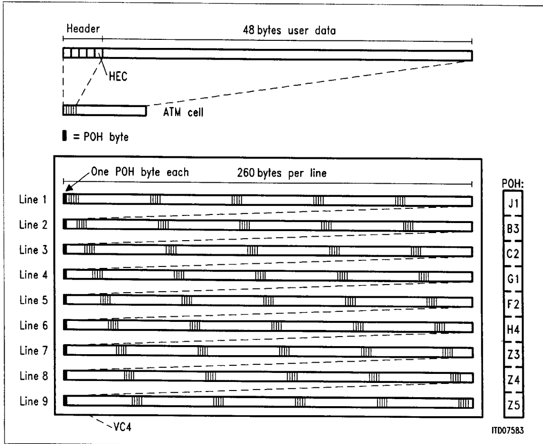
Figure 6 Virtual Container-4
