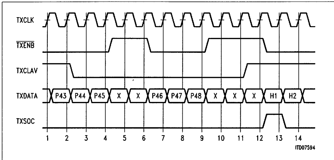
Figure 19 TxClav Example #4
