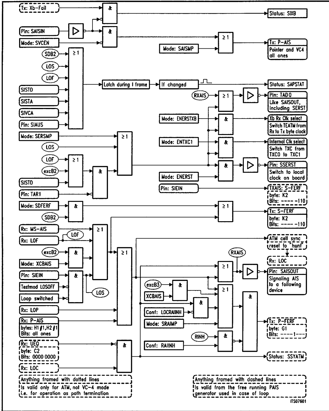
Figure 28 Alarm Handling
