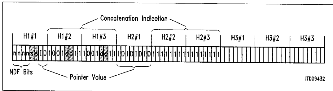
Figure 9 Structure of the AU-4 (or payload) Pointer
