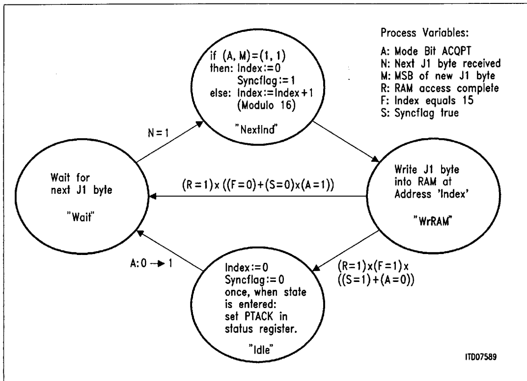
Figure 13 State Diagram of Path Trace Acquiring Algorithm
