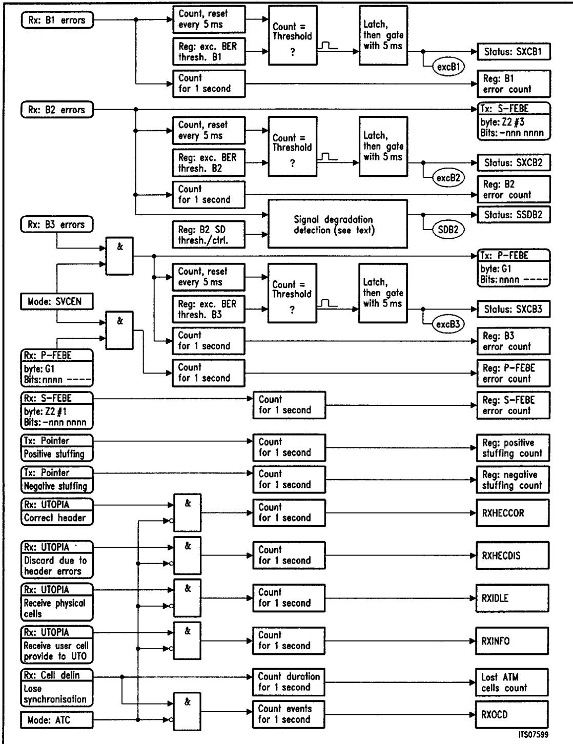
Figure 26 Performance Monitoring
