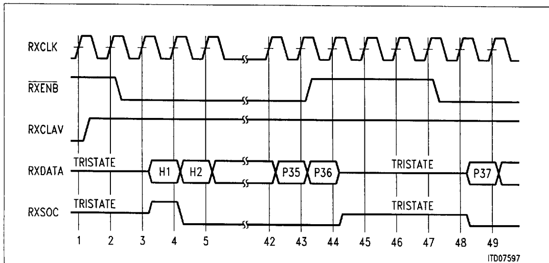
Figure 22 RxClav Example #3
