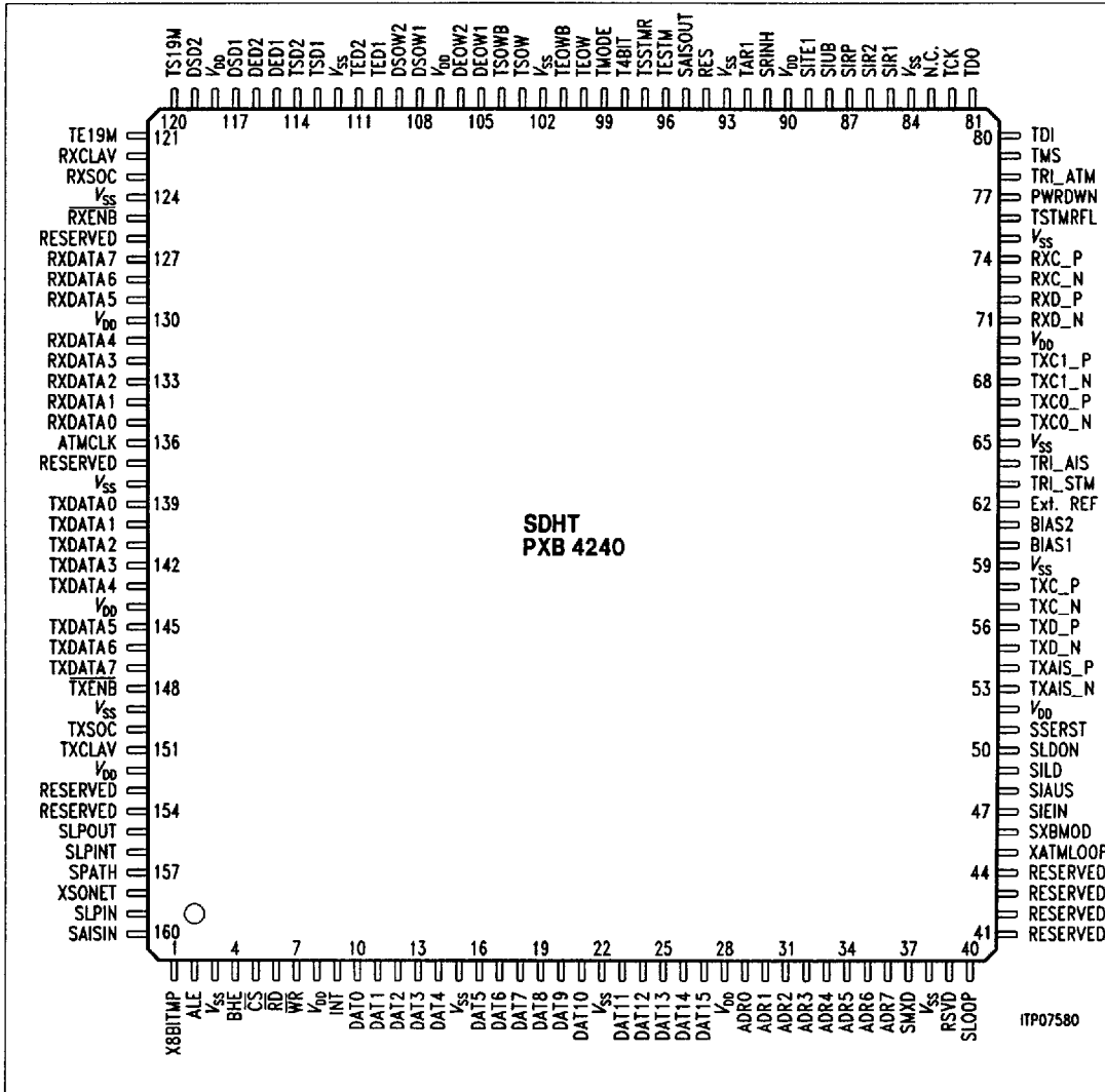
Figure 2 SDHT Pin Configuration
