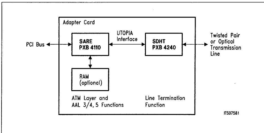
Figure 3 ATM Adapter Card Example
