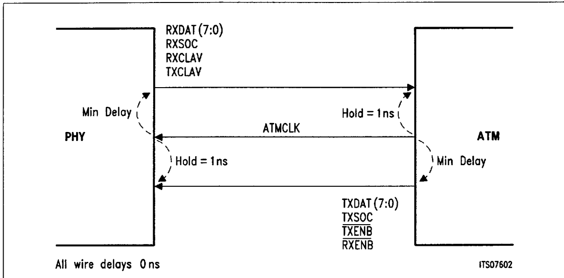
Figure 31 Timing Relationship for UTOPIA Signals
