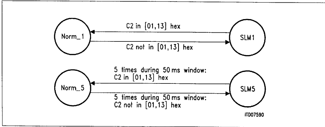
Figure 14 Signal Label Mismatch Detection
