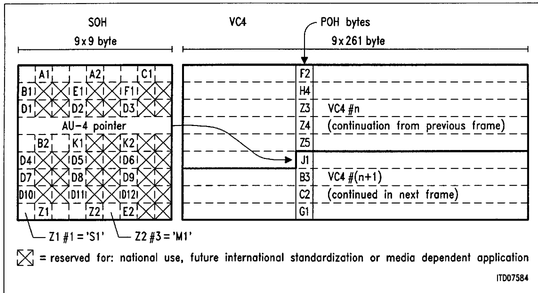
Figure 7 STM-1 Frame Structure
