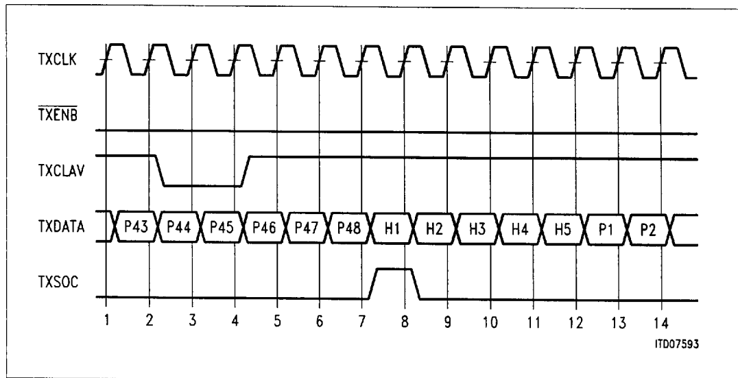
Figure 18 TxClav Example #3
