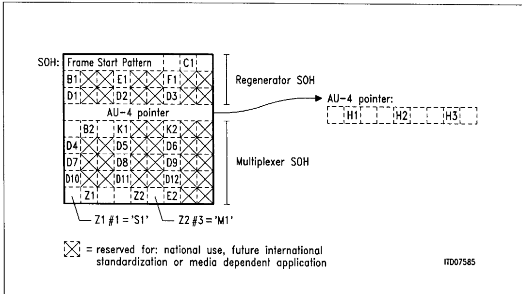
Figure 8 SOH and AU-4 Pointer
