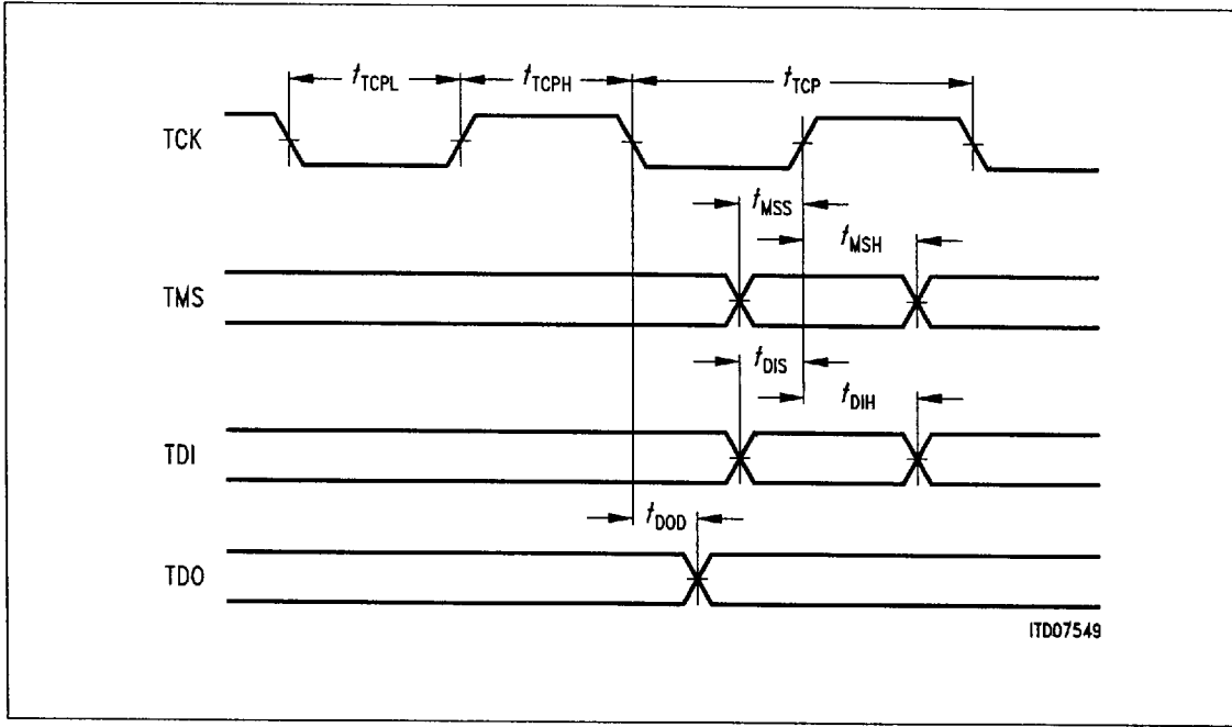
Figure 32 JTAG interface timing diagram
