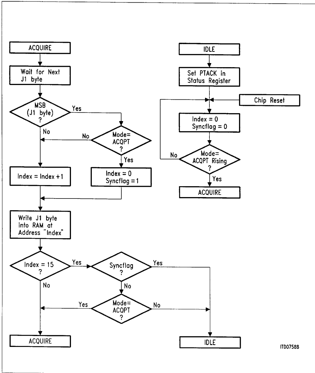
Figure 12 Flow of Path Trace Acquiring Algorithm
