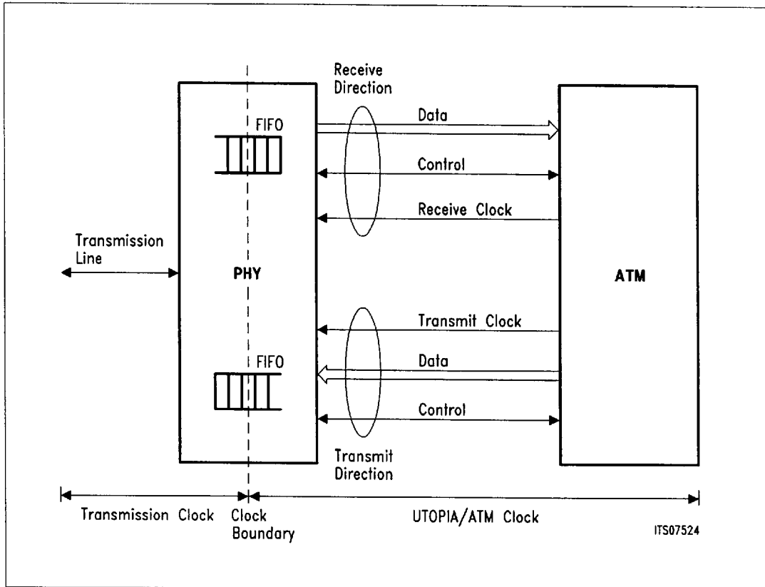
Figure 15 UTOPIA Reference Configuration
