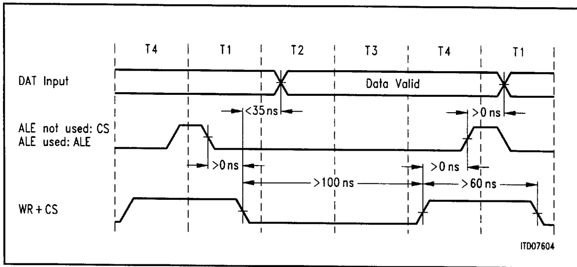
Figure 34 SDHT Write Cycle Timing (setup, hold, pulse width)
