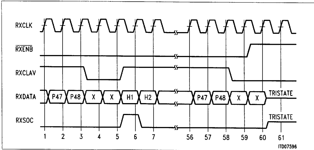
Figure 21 RxClav Example #2
