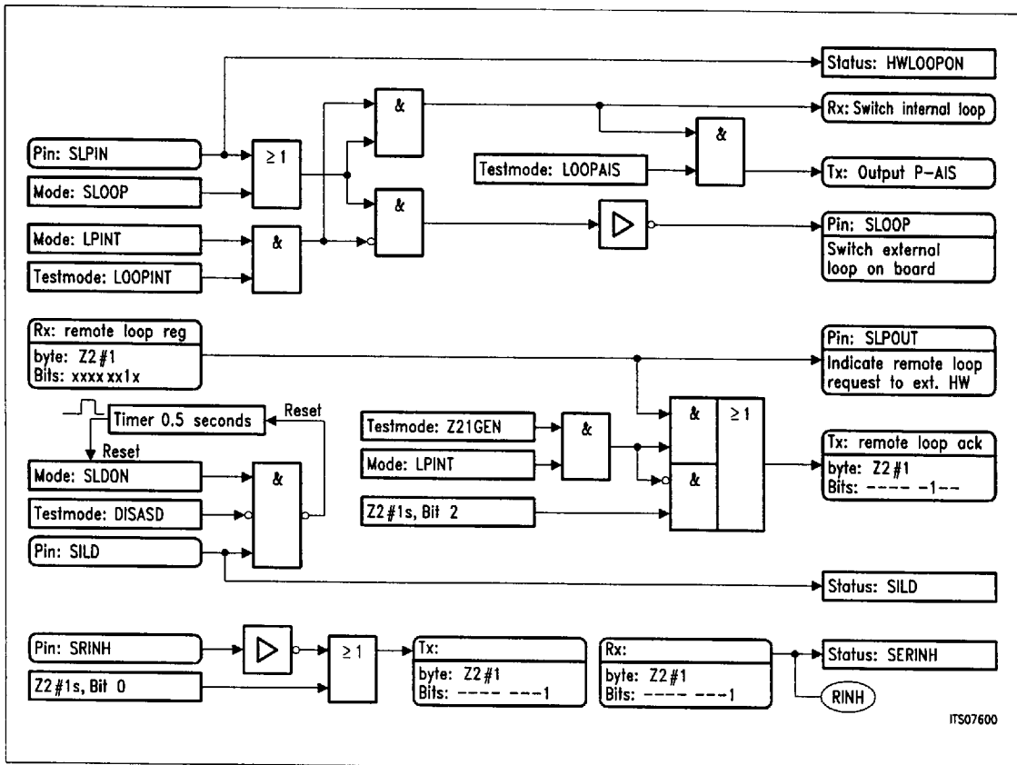
Figure 27 Special OAM Functions
