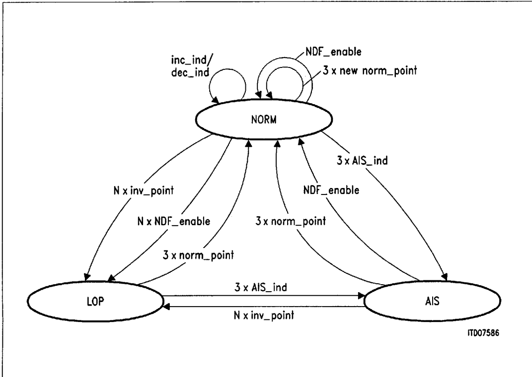
Figure 10 State Diagram of Pointer Evaluation, Normal
