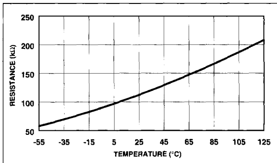
Figure 1. TC623 Sense Resistors vs. Trip Temperature
