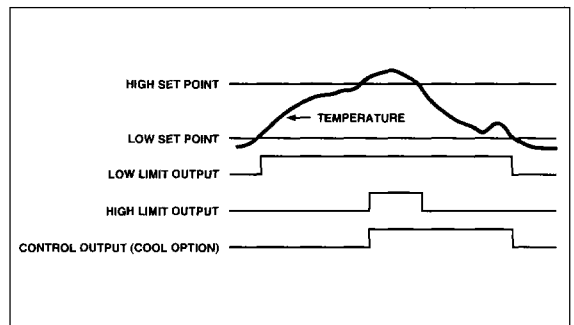
Figure 2. TC623 Temperature vs. Output
