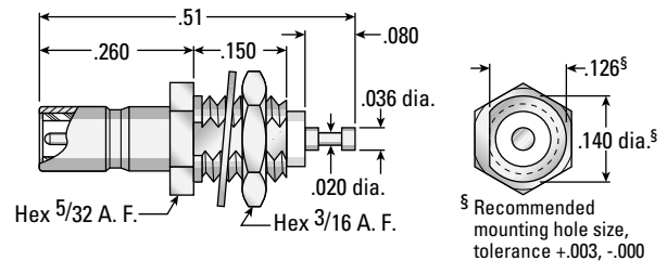
Front mount
