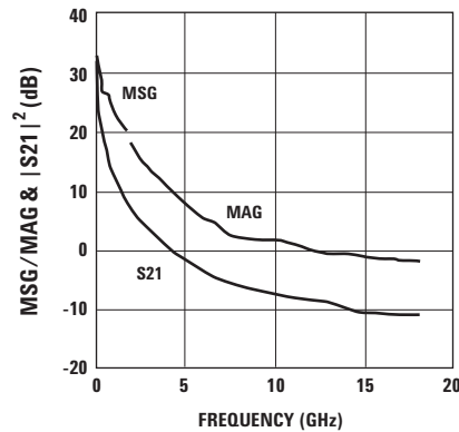
Figure 33. MSG/MAG & |S_{21}|^2 (dB) @ 4.5V, 200 mA.
