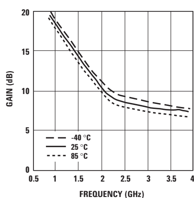
Figure 30. Gain vs. Temp and Freq.
