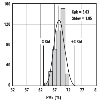
Figure 5. PAE LSL = 52, Nominal = 68.9.
