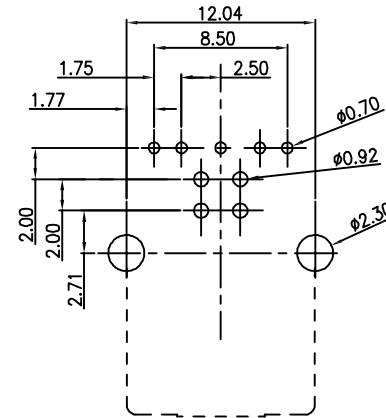
PCB LAYOUT (T=1.60mm)
