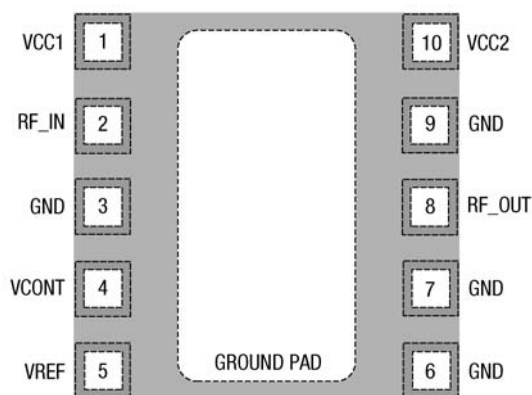
Figure 13. CX77112 Pin Configuration
