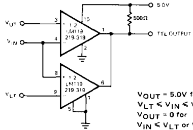
Window Detector
