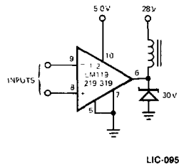
Relay Driver
