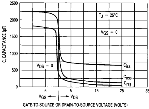
Figure 11. Capacitance Variation
