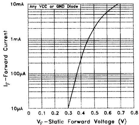
Low I_F vs V_F Characteristic
